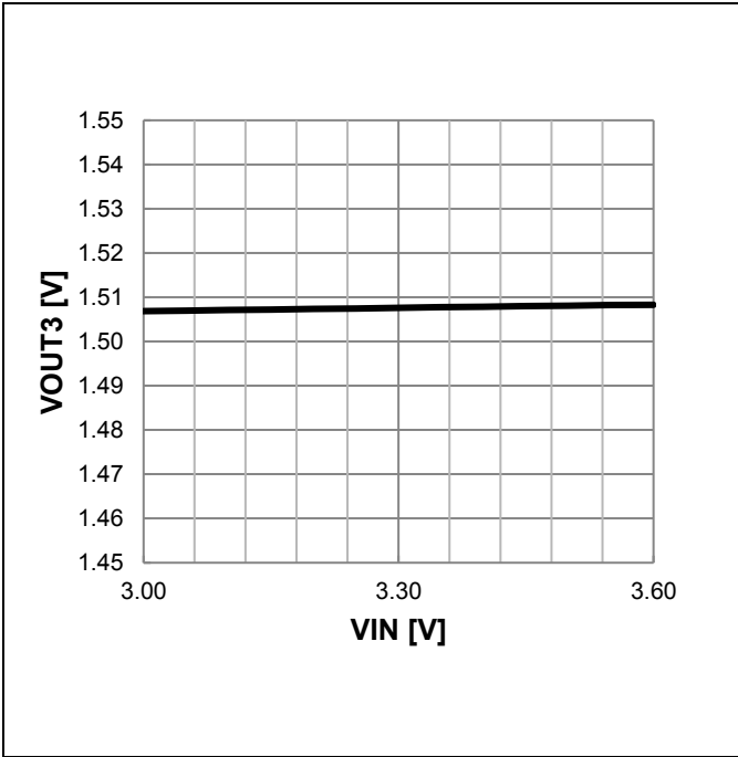
Figure 42. VOUT3 Output Voltage vs VIN (VOUT3 = 1.5 V Setting)
