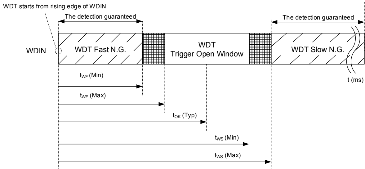
Figure 34. WDT Function
