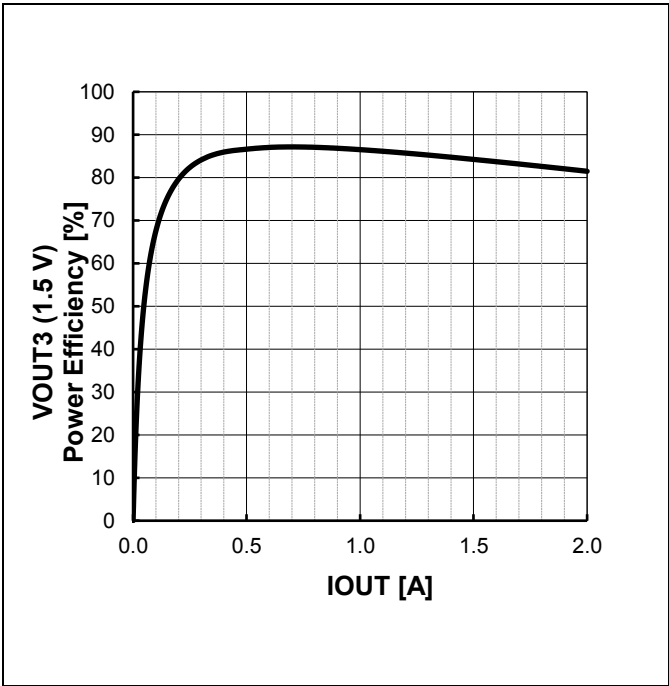
Figure 54. VOUT3 Power Efficiency vs IOUT (VOUT3 = 1.5 V Setting)
