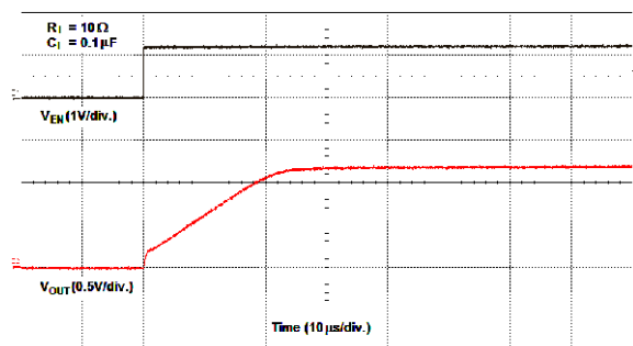
Fig. 23 - Turn-On Time ( V_{IN} = 1.2\text{ V} )
