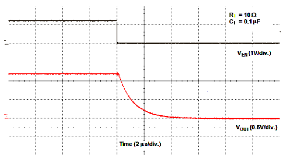
Fig. 24 - SiP32451 and SiP32452 Turn-Off Time ( V_{IN} = 1.2\text{ V} )
