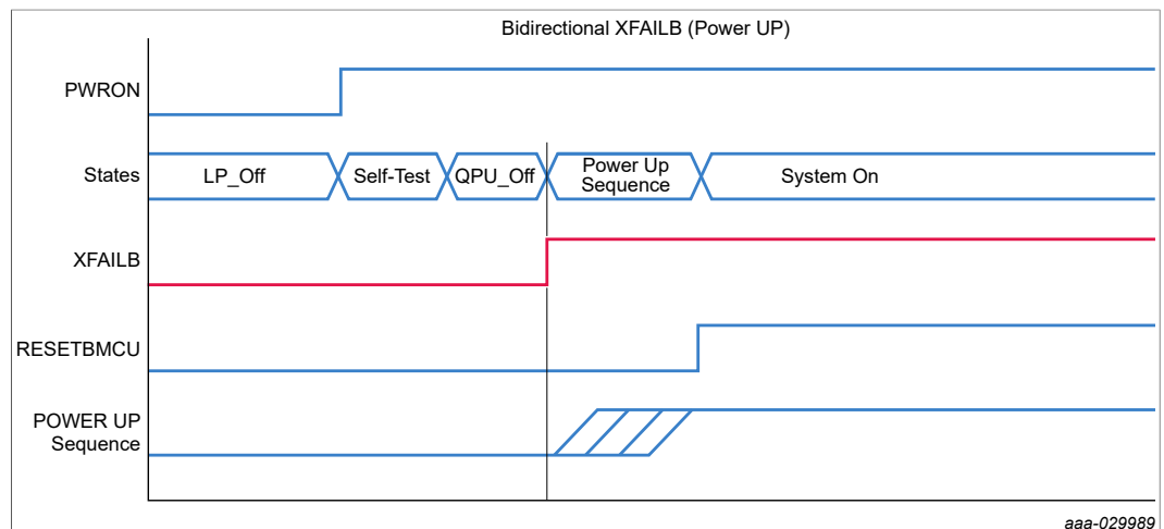
Figure 16. XFAILB behavior during a power up sequence
