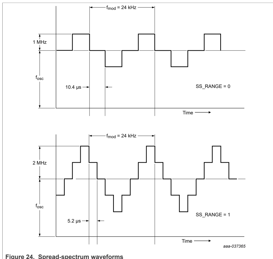
Figure 24. Spread-spectrum waveforms
