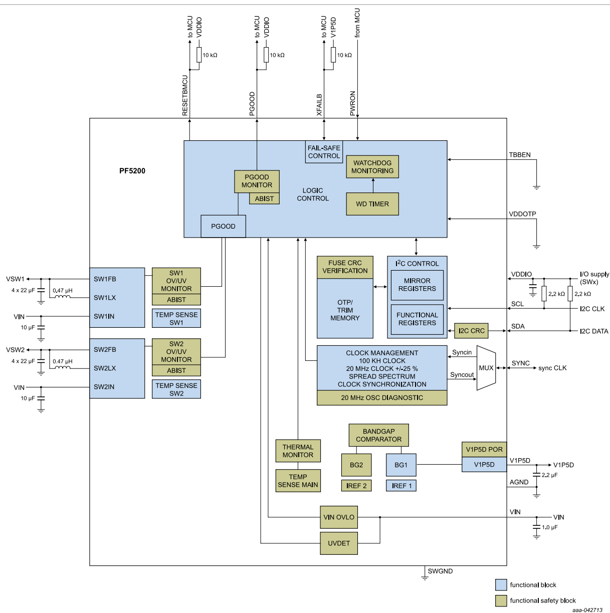
Figure 29. Typical application diagram
