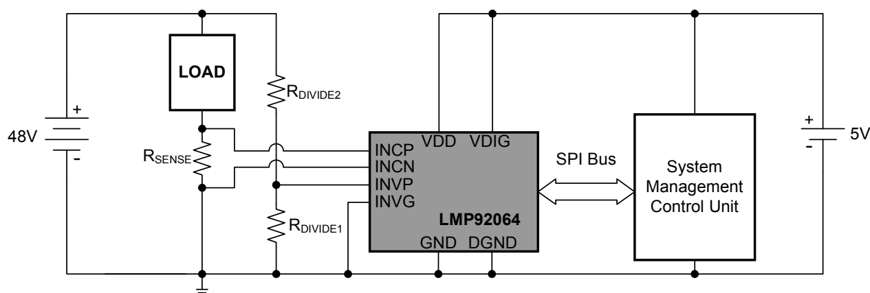
Simplified Schematic
