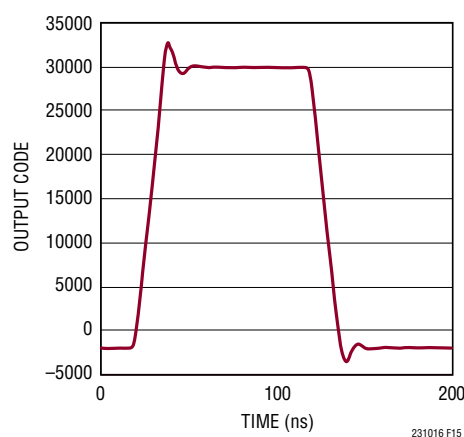
Figure 15. Transient Response of the LTC2310-16
