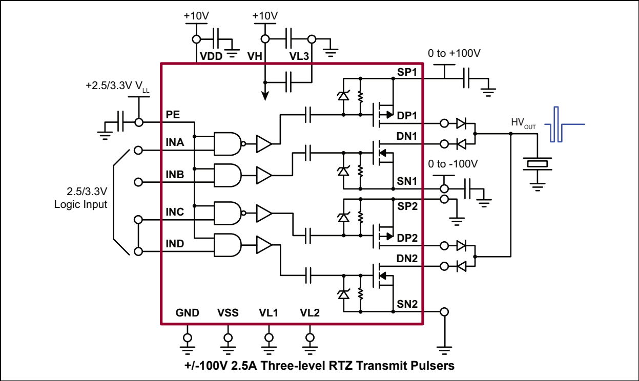
HV7361 Typical Application Circuit
