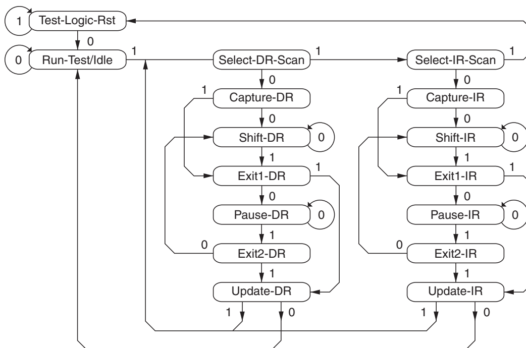
Figure 39. TAP States
