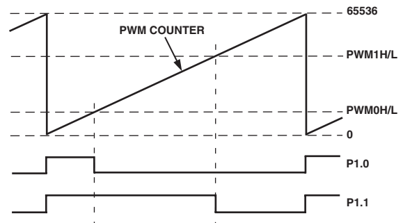
Figure 29. PWM Mode 3
