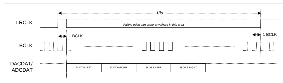
Figure 54 TDM in DSP Mode A
