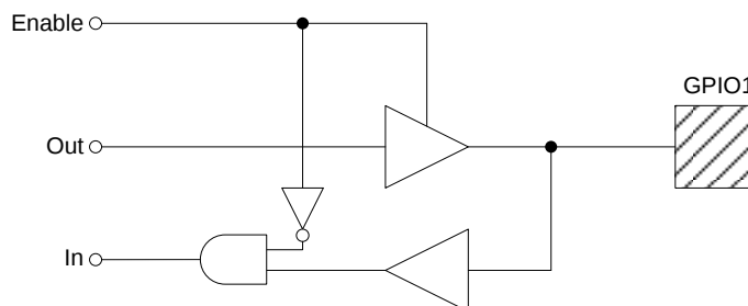
Figure 36 GPIO Pad
