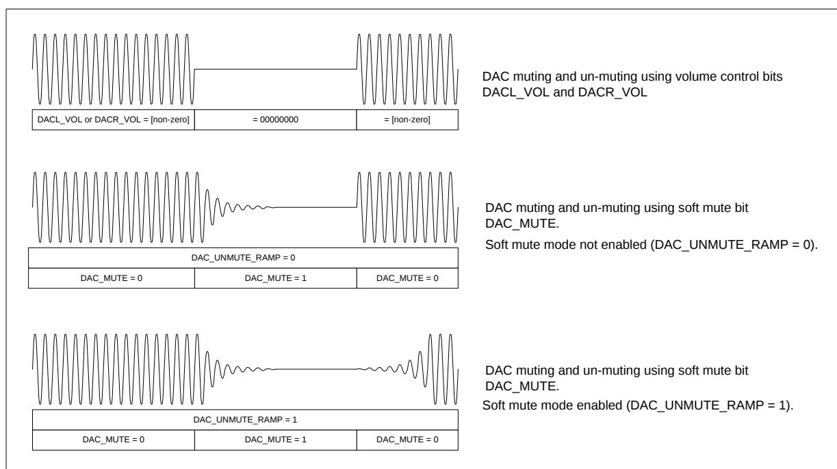
Figure 21 DAC Soft Mute Control
