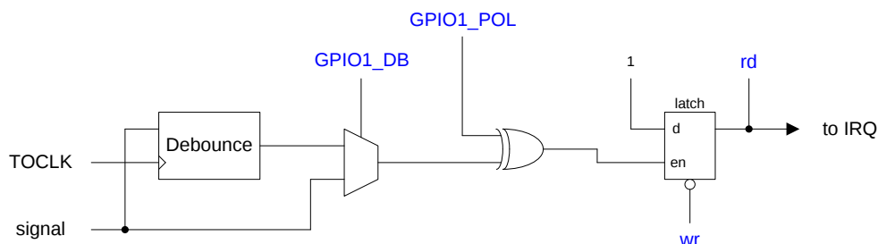
Figure 37 GPIO Function
