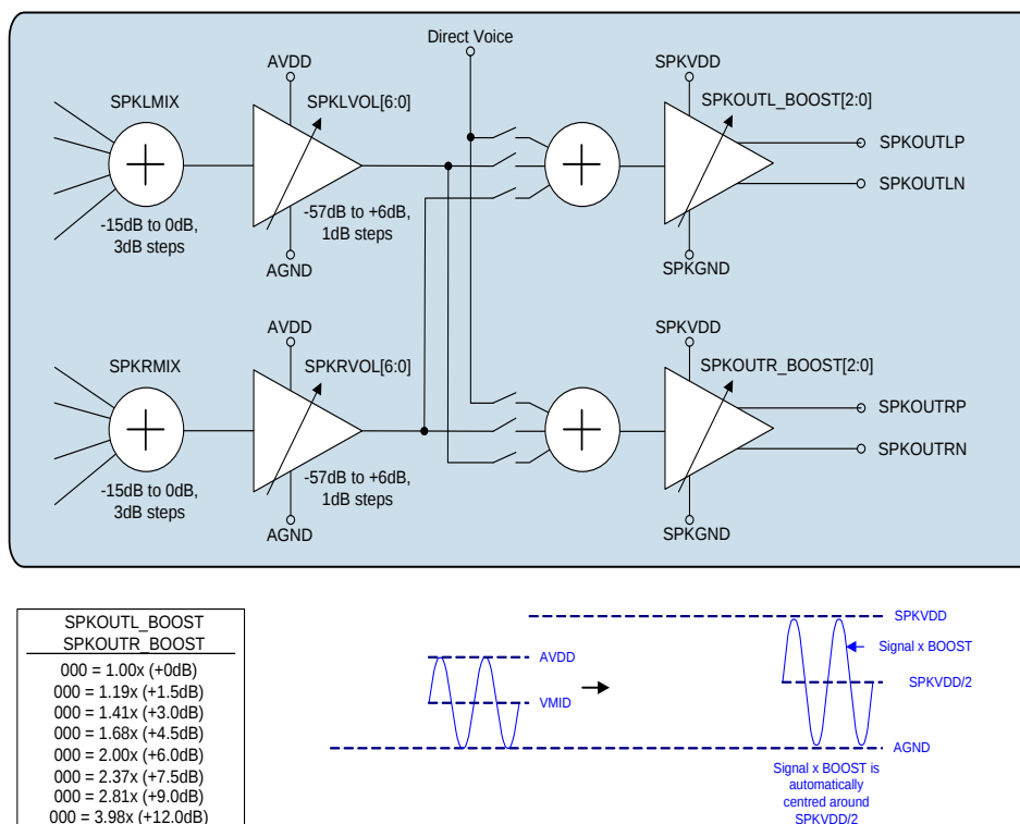
Figure 26 Speaker Output Configuration and AC Boost Operation
