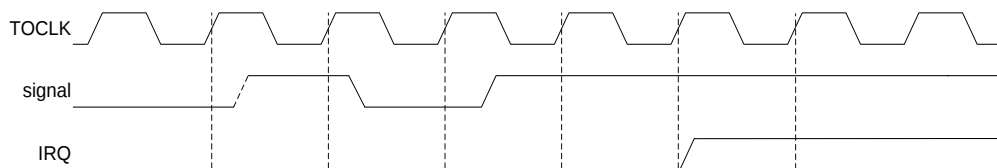
Figure 35 GPIO De-bounce
