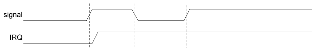
Figure 34 GPIO Latch
