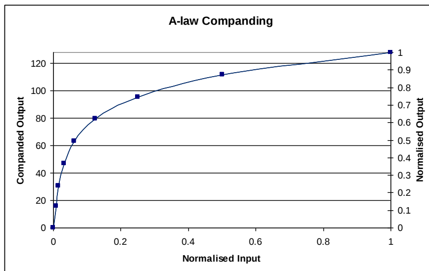
Figure 58 A-Law Companding
