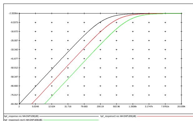
Figure 74 ADC Digital High Pass Filter Ripple (48kHz, Voice Mode, ADC_HPF_CUT=01, 10 and 11)
