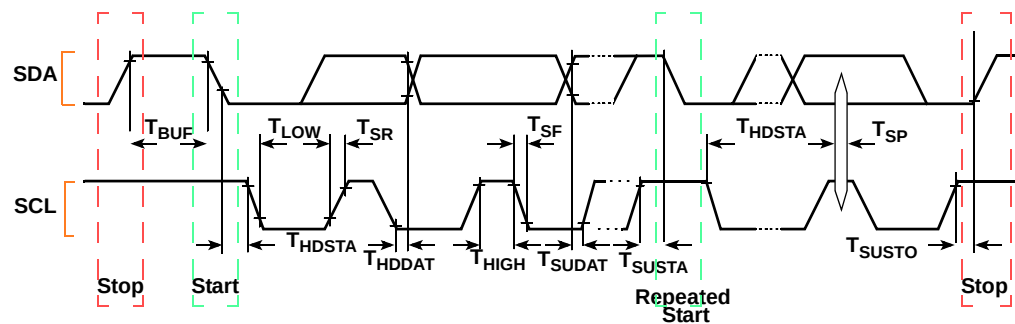
Figure 60: I 2 C Interface Signal Timings
