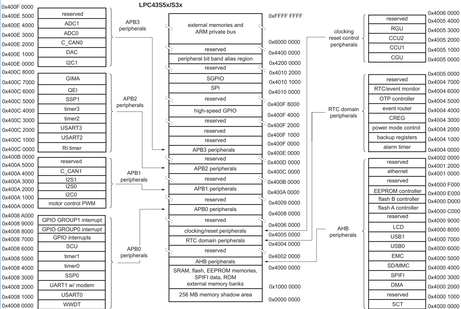
Fig 8. LPC43S5x/S3x Memory mapping (peripherals)
