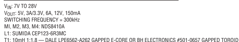
Figure 12. LTC3707-SYNC High Efficiency Low Noise 5V/3A, 3.3V/5A, 12V/120mA Regulator
