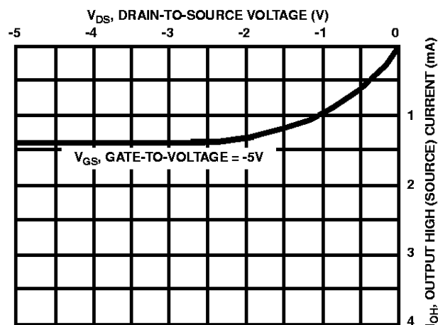
FIGURE 20. CDP1802BC MINIMUM OUTPUT HIGH (SOURCE) CURRENT CHARACTERISTICS
