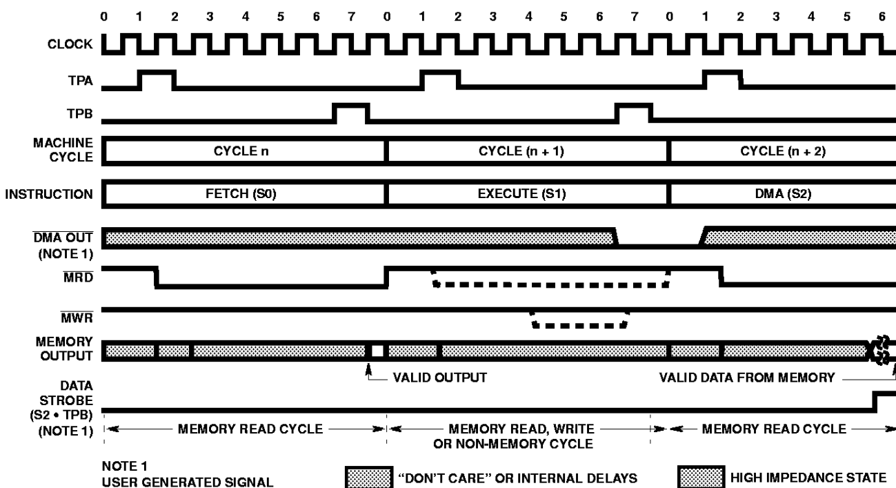
FIGURE 13. DMA OUT CYCLE TIMING WAVEFORMS
