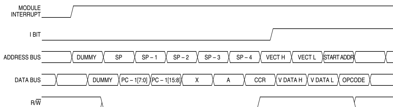
Figure 13-9. Interrupt Entry
