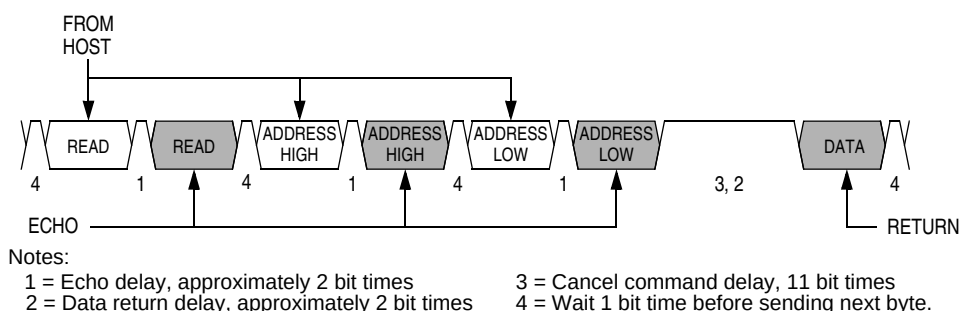
Figure 15-16. Read Transaction
