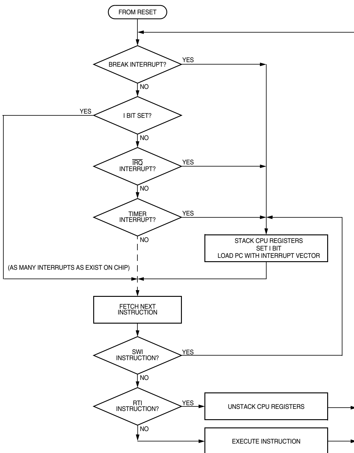
Figure 13-8. Interrupt Processing
