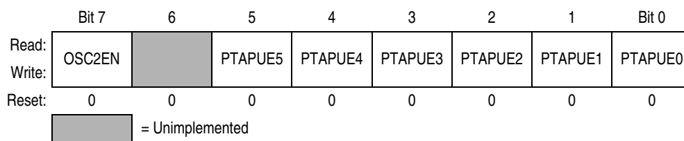
Figure 12-5. Port A Input Pullup Enable Register (PTAPUE)
