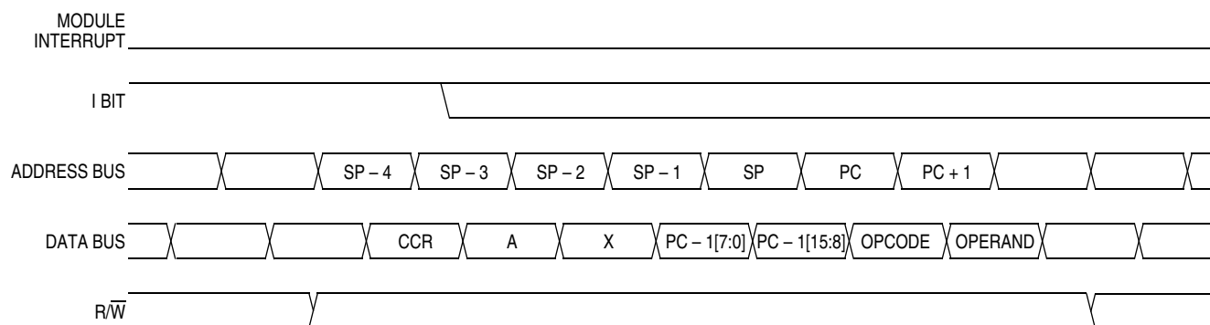
Figure 13-10. Interrupt Recovery
