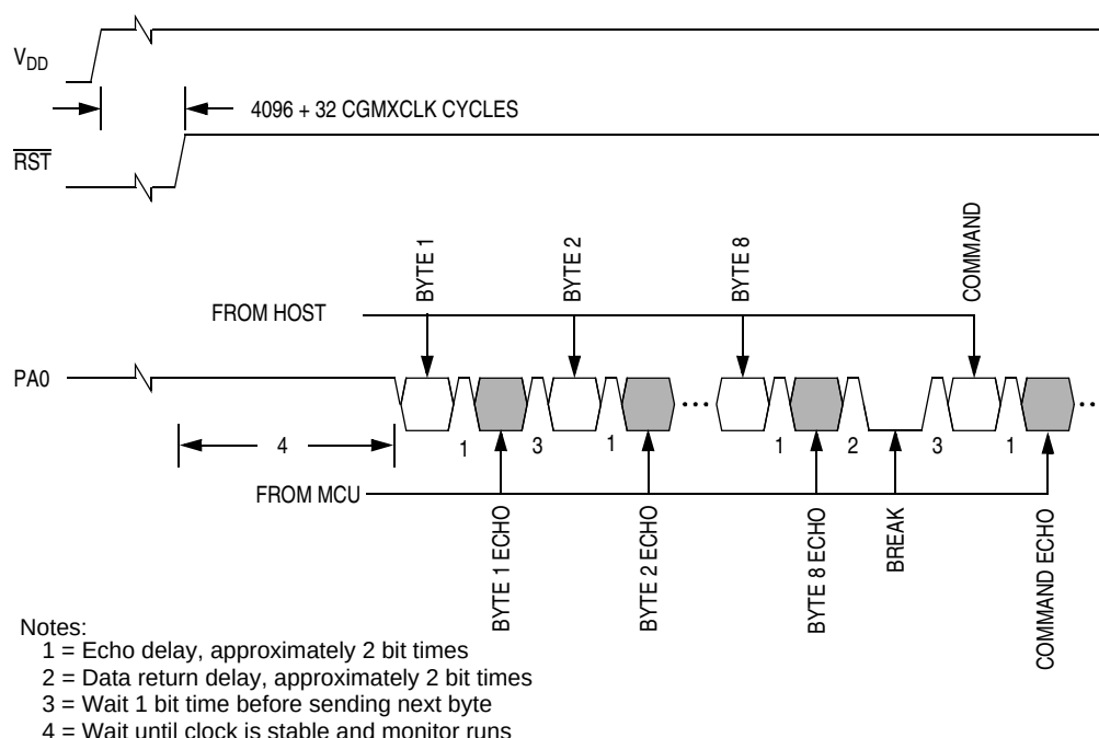
Figure 15-19. Monitor Mode Entry Timing
