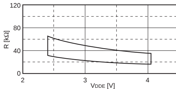
Pull-down resistor example characteristics Ta = + 25 °C
