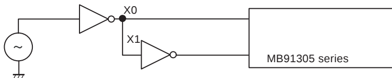
Example of using external clock (normal)
