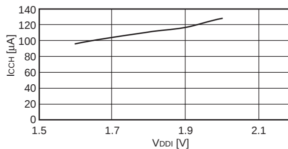
ICCH-VDD I example characteristics Ta = + 25 °C
