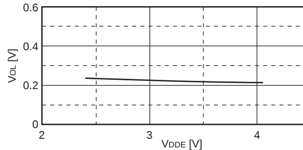
V_{OL} - V_{DDE} example characteristics
