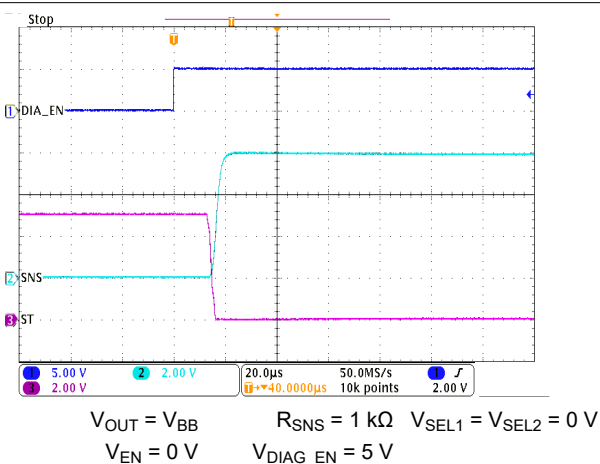
Figure 7-31. Open Load Detection Time ( t_{OL2} ) on Rising DIA\_EN
