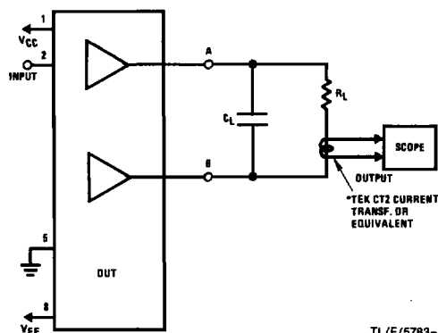
FIGURE 1. Differential Connection
