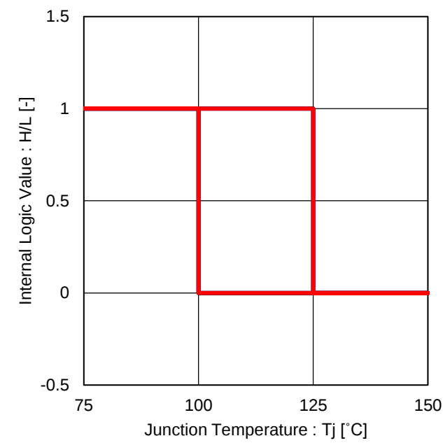
Figure 43 Thermal Shutdown
