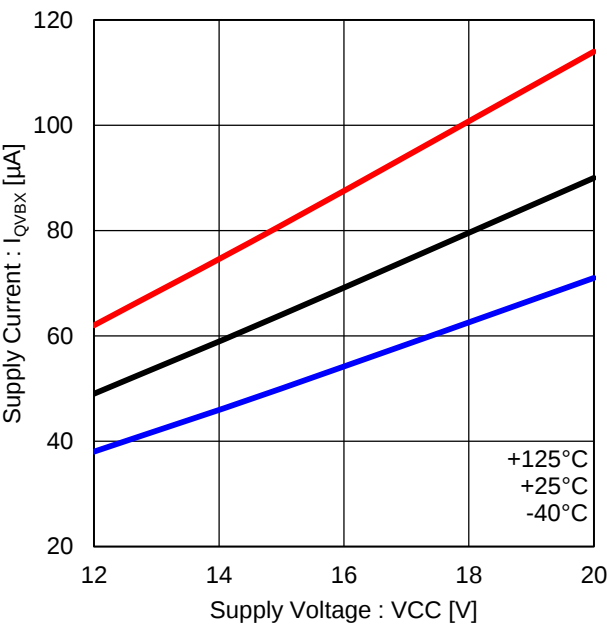
Figure 16. Quiescence Current (High Side Driver, Each Phase)
