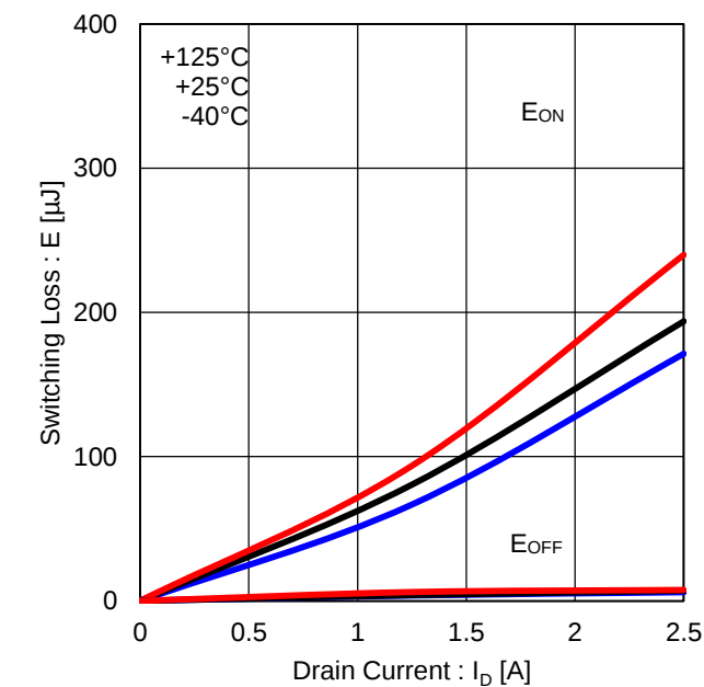
Figure 24. Low Side Switching Loss (VDC=300V)
