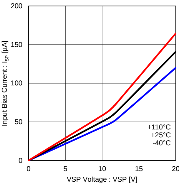
Figure 29. VSP Input Bias Current
