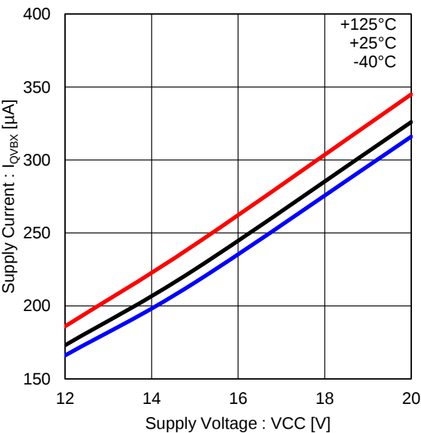
Figure 17. High Side Driver Operating Current (f PWM : 20kHz, Each Phase)
