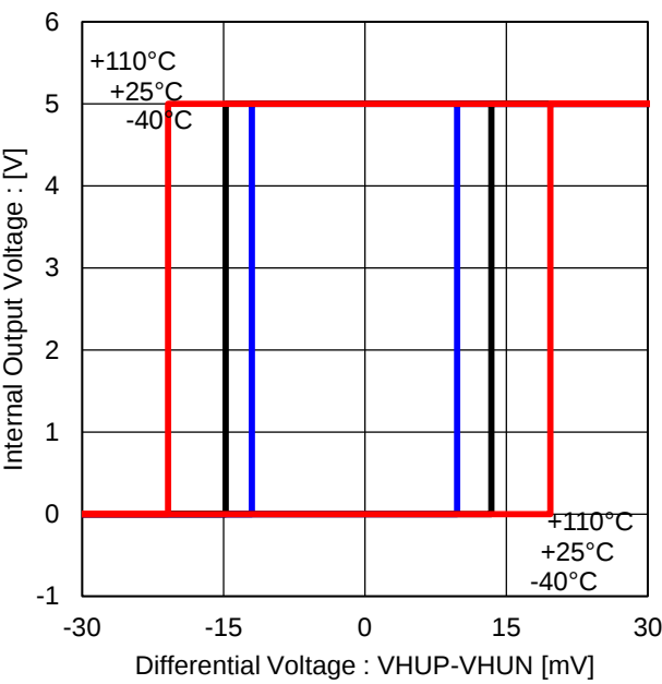
Figure 28. Hall Comparator Hysteresis Voltage
