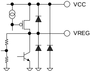
Figure 53. VREG, VCC
