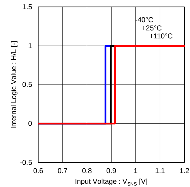
Figure 42. OCP Input Threshold Voltage (SNS)
