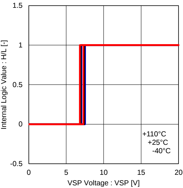
Figure 31. Testing Mode Threshold Voltage
