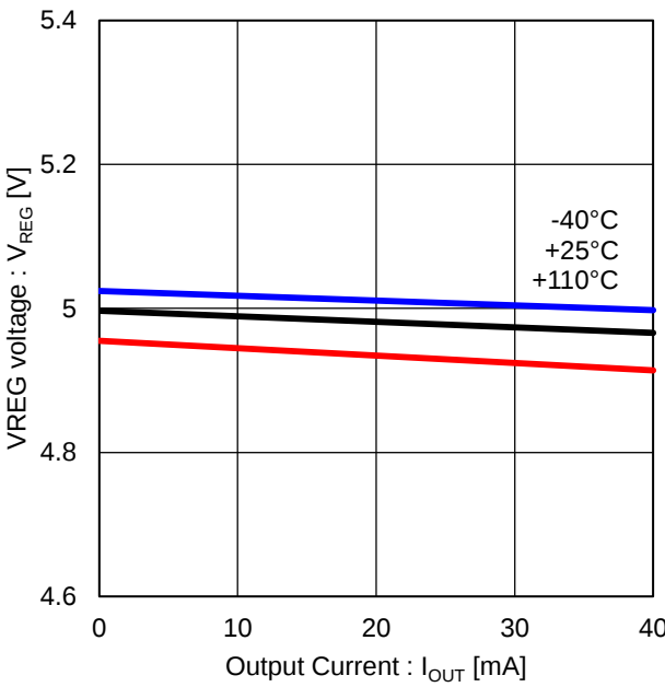
Figure 27. VREG Drive Capability
