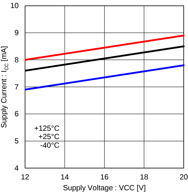
Figure 15. Low Side Drivers Operating Current (F PWM : 20kHz)
