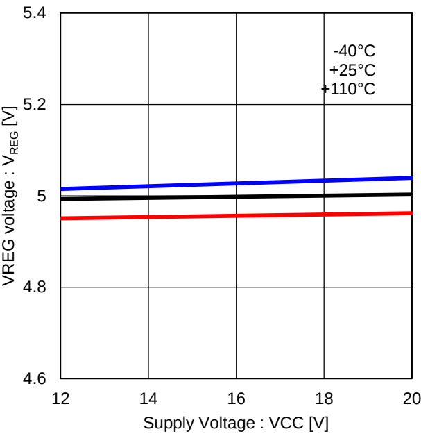
Figure 26. VREG vs VCC
