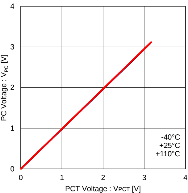
Figure 33. PCT vs PC Linearity (R PCT =R PC =100kΩ)
