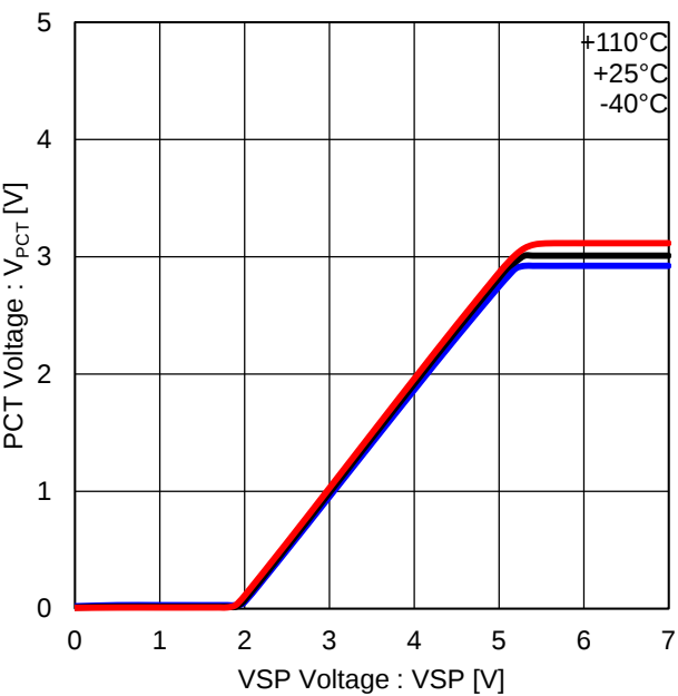
Figure 32. VSP vs PCT Offset Voltage
