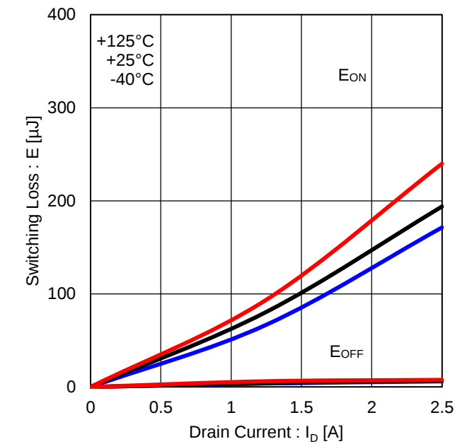
Figure 22. High Side Switching Loss (VDC=300V)
