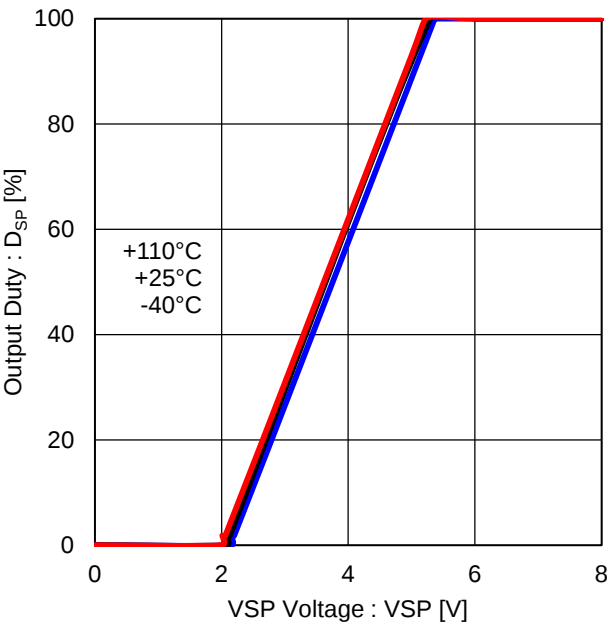
Figure 30. Output Duty vs VSP Voltage
