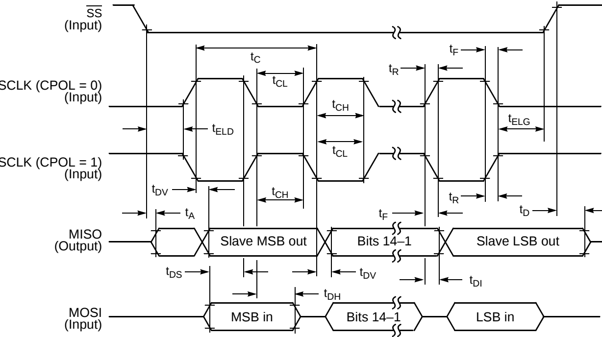
Figure 10-12 SPI Slave Timing (CPHA = 1)
