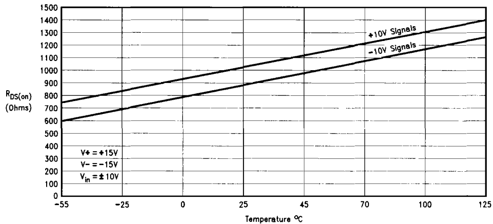
Figure 13: Typical R_{DS(ON)} Variation with Temperature
