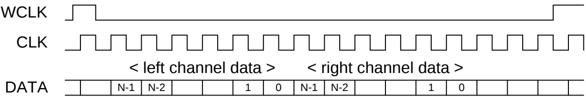
Figure 36: DSP Format
