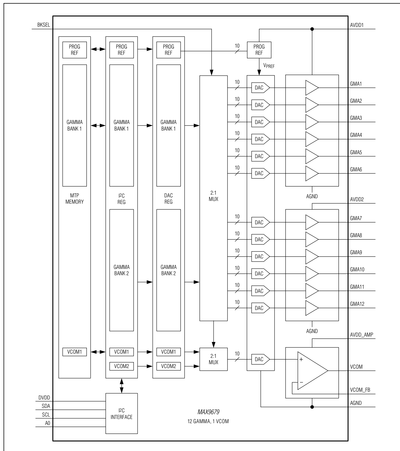
Functional Diagram
