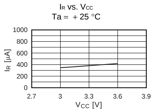
A/D converter reference power supply current at stop
