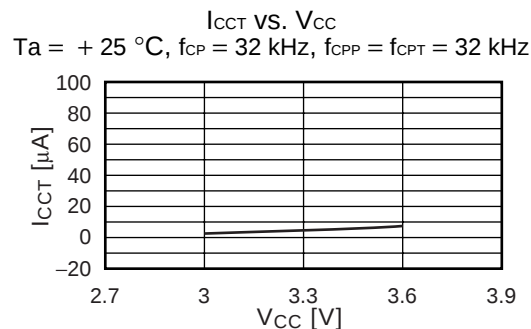
Watch mode power supply current
