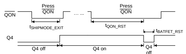
Figure 2. \overline{\text{QON}} Timing
