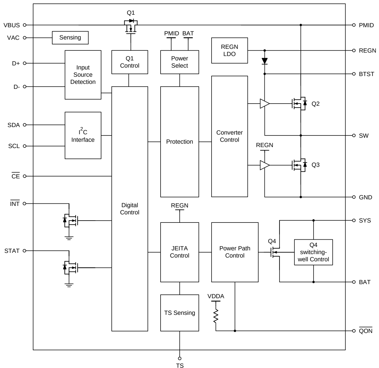
RT9471D Functional Block Diagram
