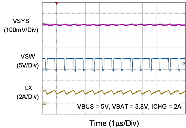
Buck Switching
