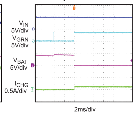
Short Circuit
