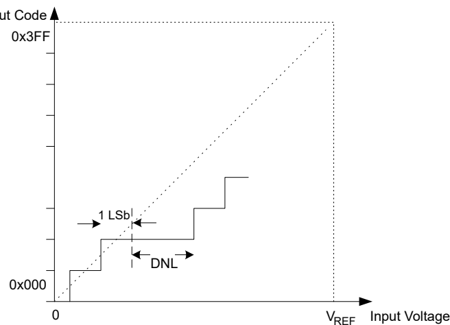
Figure 5-4. Differential Nonlinearity
