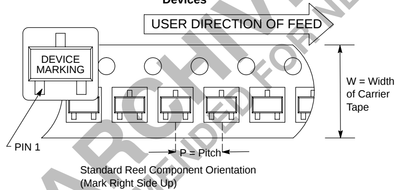
Tape &amp; Reel Specifications Table
