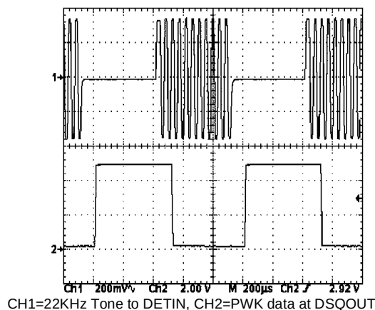
Figure 8: DETIN/DSQOUT Waveform
