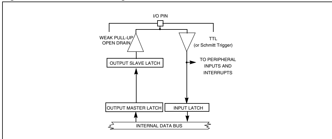
Figure 82. Bidirectional configuration
