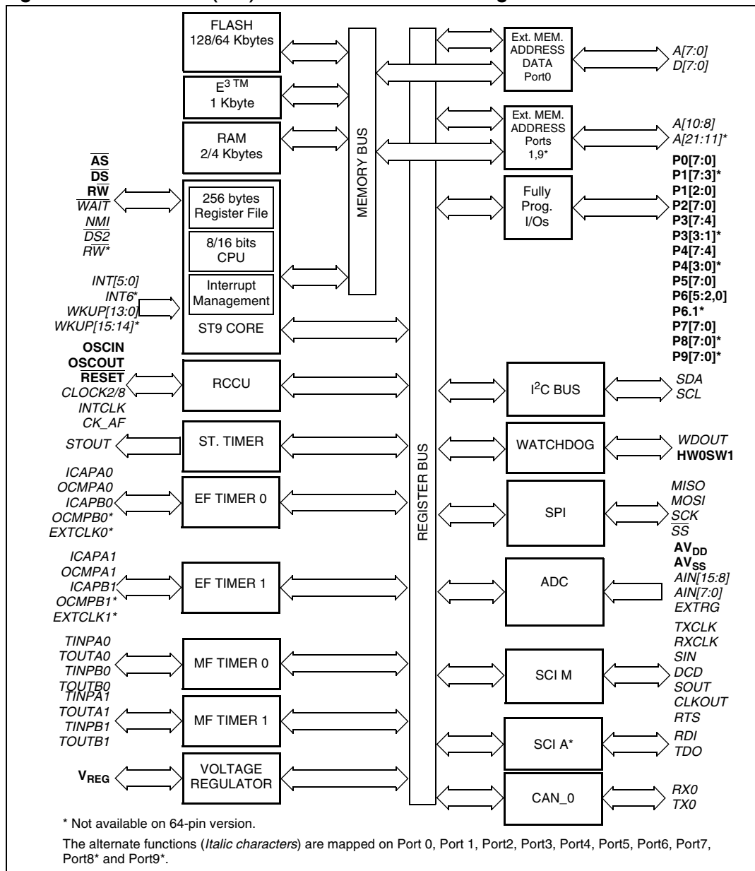
Figure 3. ST92F150C(R/V)1/9: Architectural block diagram
