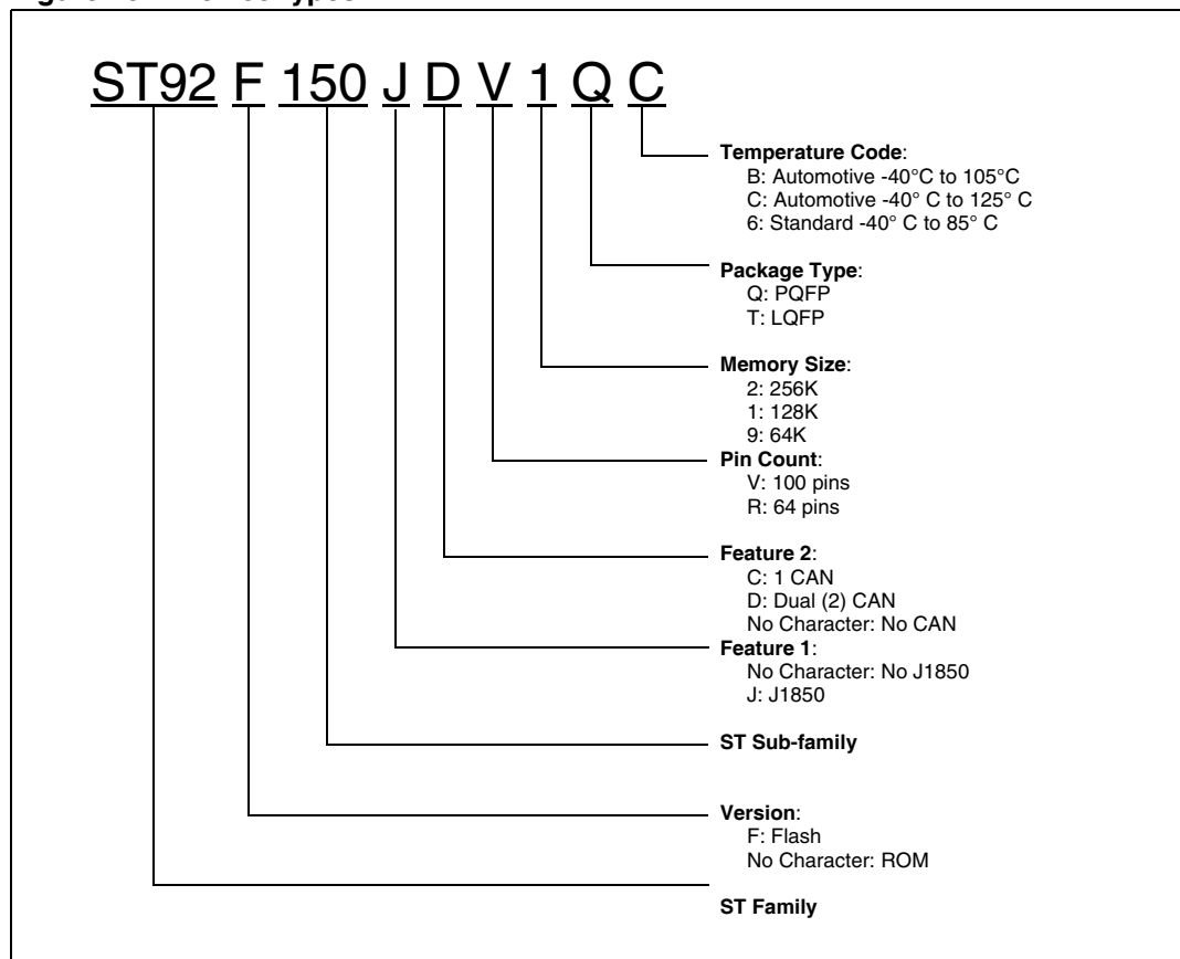
Figure 197. Device types
