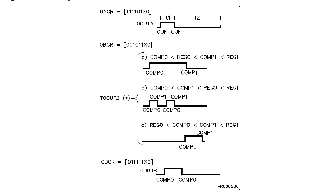
Figure 118. Sample waveforms
