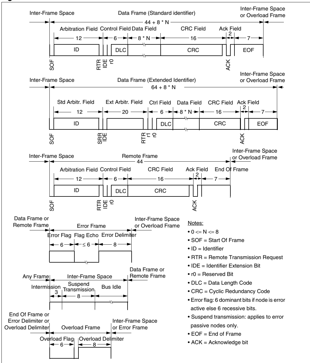
Figure 167. CAN frames
