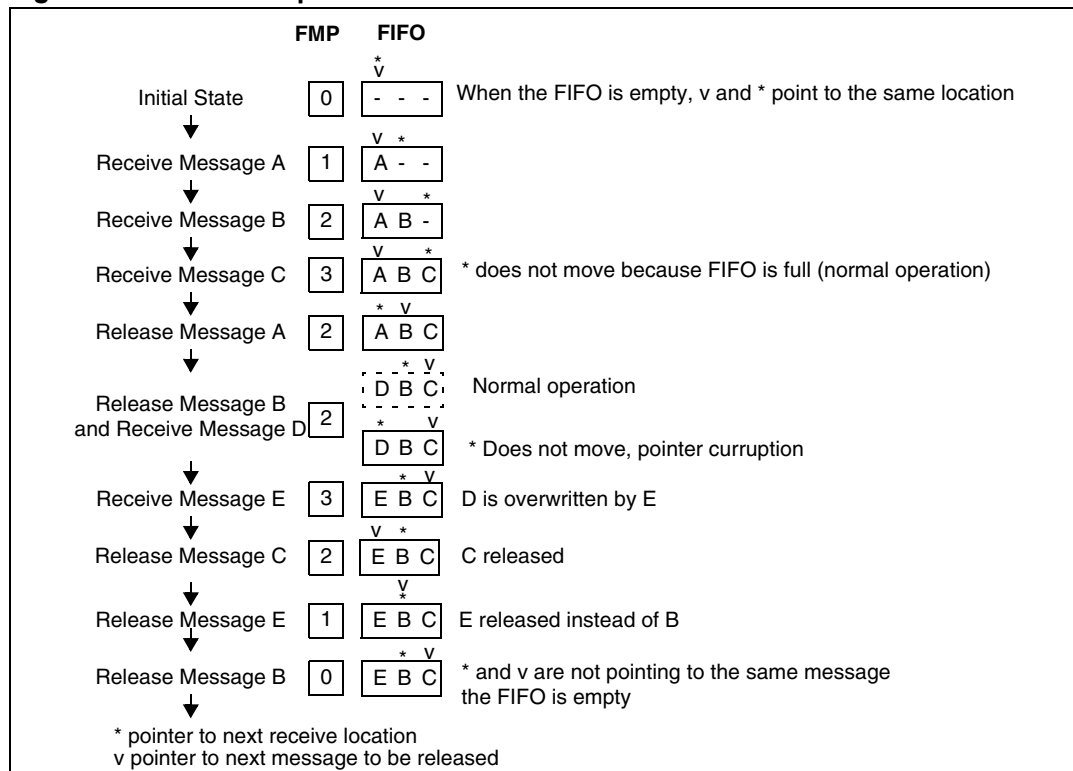
Figure 202. FIFO corruption
