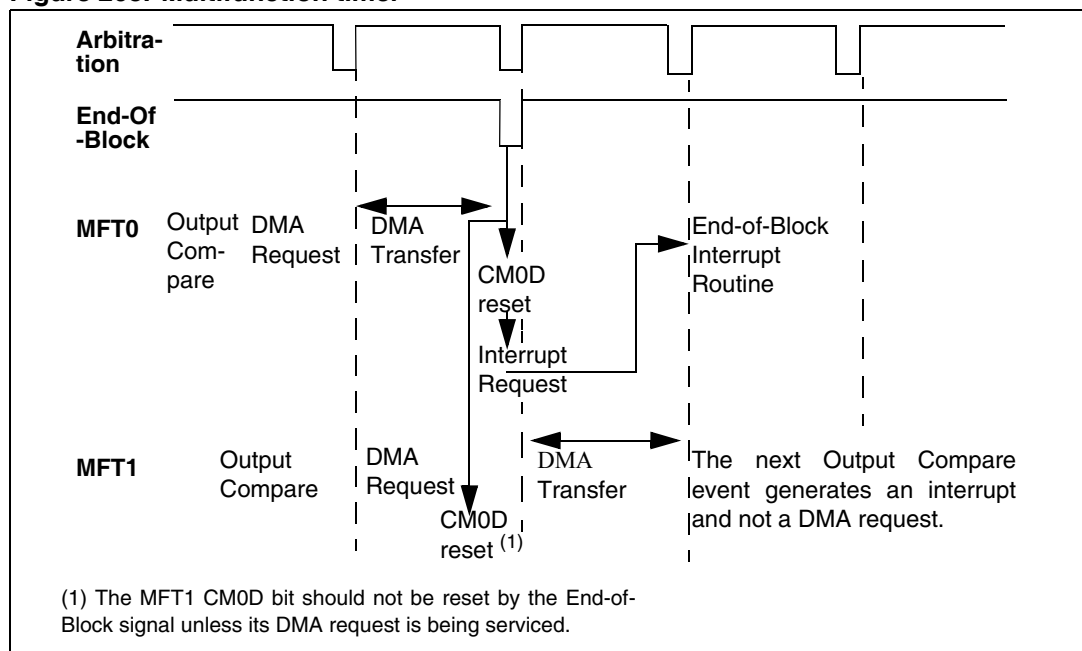
Figure 208. Multifunction timer
