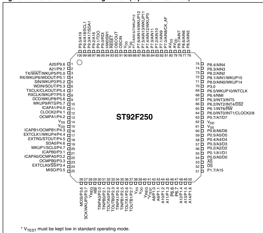
Figure 15. ST92F250: Pin configuration (top-view LQFP100)
