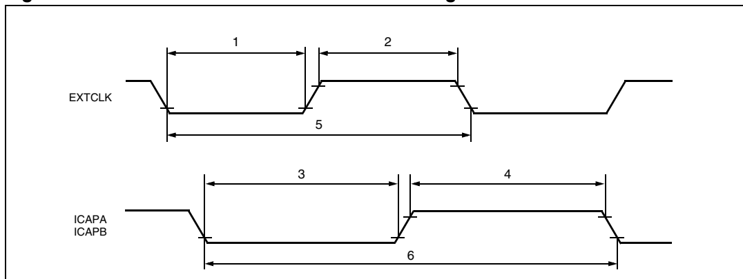
Figure 182. Extended function timer external timing
