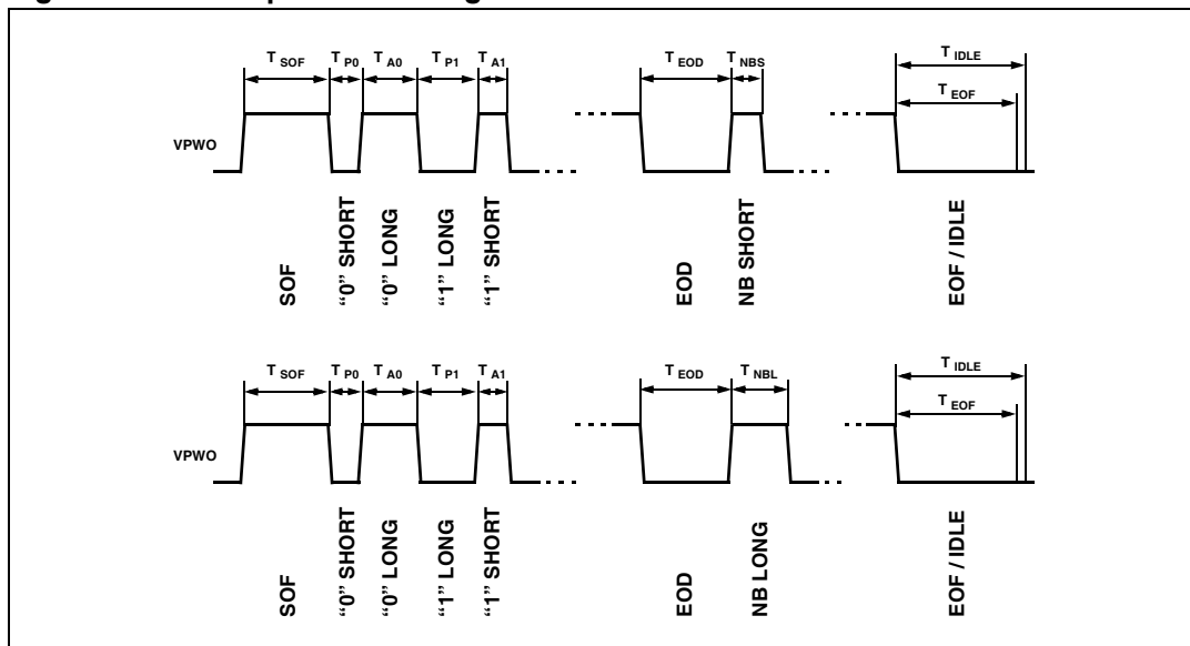
Figure 194. J1850 protocol timing
