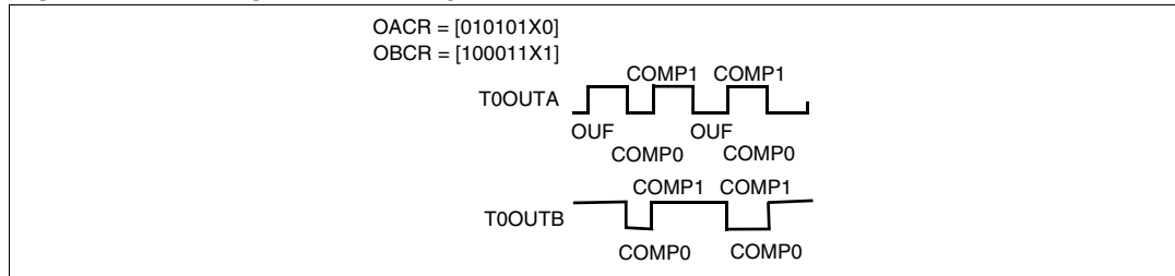
Figure 115. Configuration example 1
