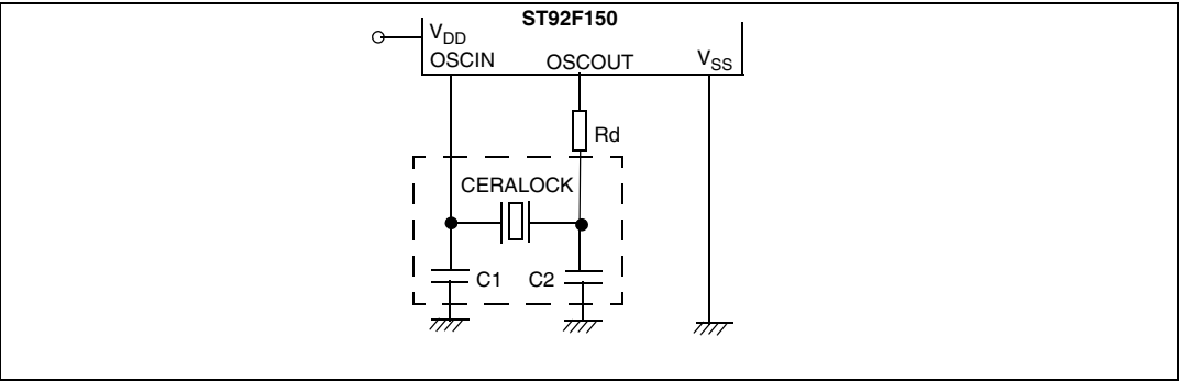
Figure 69. Test circuit
