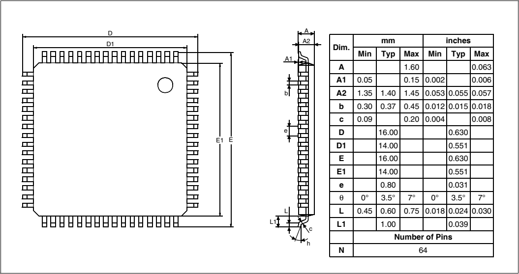
Figure 198. 64-pin low profile quad flat package
