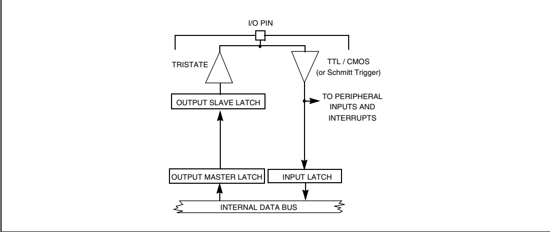
Figure 80. Input configuration
