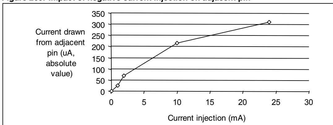
Figure 209. Impact of negative current injection on adjacent pin
