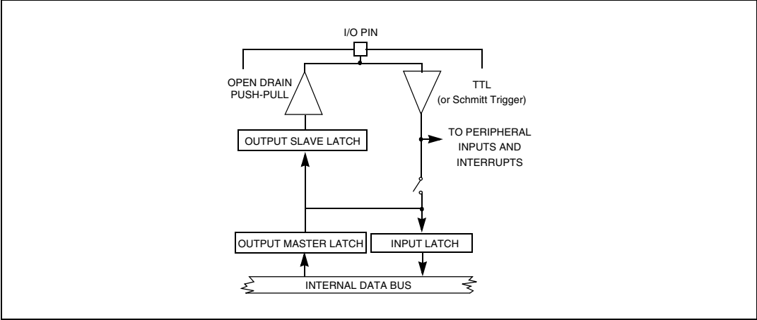
Figure 81. Output configuration
