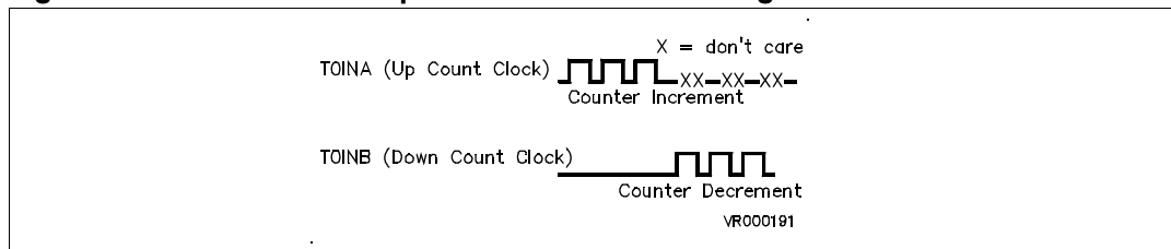
Figure 108. TxINA = Clock Up - TxINB = Clock down signal
