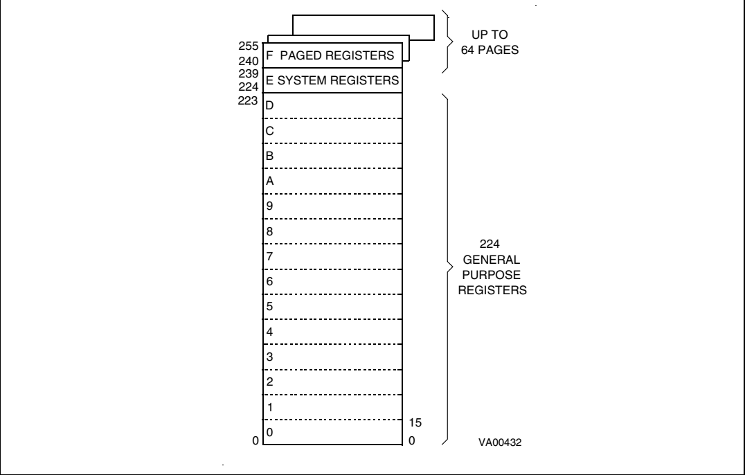
Figure 19. Register groups
