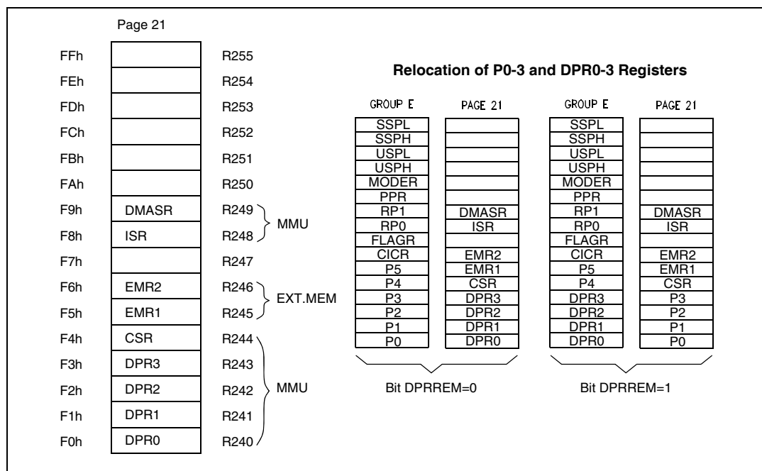
Figure 73. Page 21 registers
