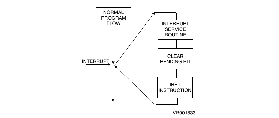
Figure 44. Interrupt response
