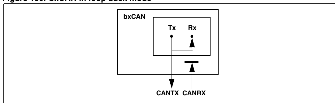
Figure 159. bxCAN in loop back mode
