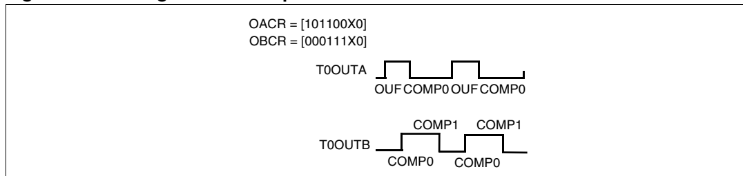
Figure 117. Configuration example 3
