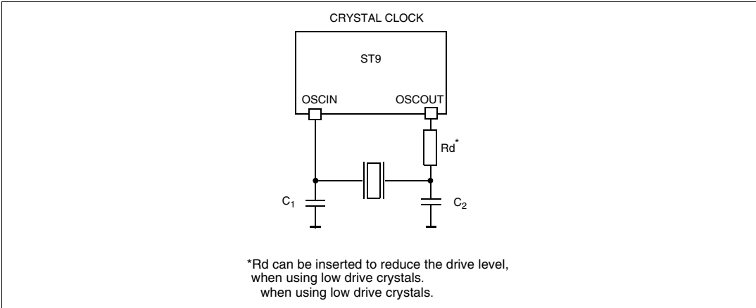
Figure 66. Crystal oscillator
