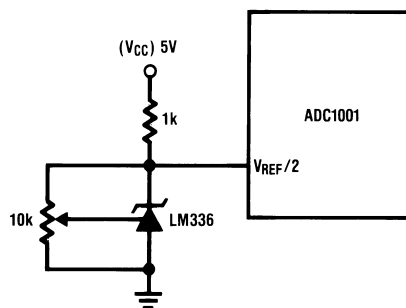
FIGURE 2. Full-Scale Adjust
