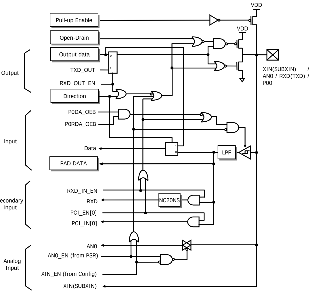
Figure 1.18 XIN(SUBXIN) / AN0 /RXD /P0[0] Port Structure
