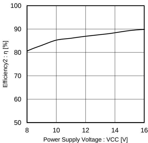
Figure 10. Efficiency 2 vs Power Supply Voltage ( R_{RT} = 4 \text{ k}\Omega , R_{SET} = 15.1 \text{ k}\Omega , Number of LED Series = 10, Number of LED Parallels = 4)
