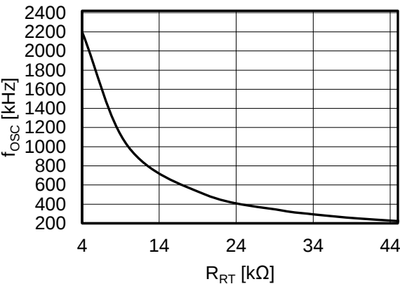
Figure 19. f OSC vs R RT
