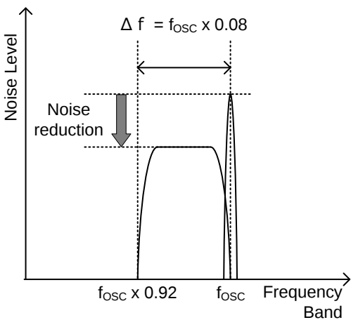
Figure 23. Spread Spectrum Function
