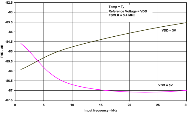
Figure 16.. THD vs Input Frequency
