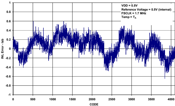
Figure 13 INL VDD= 5.5
