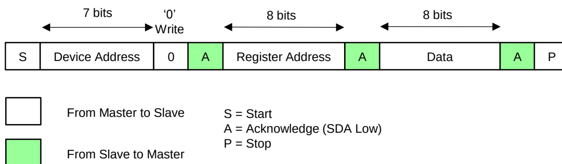
Figure 6. I 2 C Write Cycle
