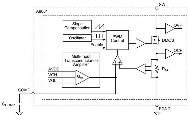
Figure 6. Boost controller circuit
