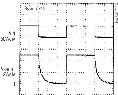
START-UP TRANSIENT
