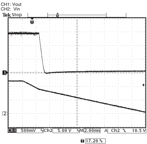
POWER-DOWN, 40A LOAD
