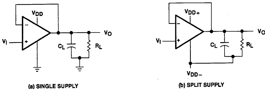
Figure 1. Unity-Gain Amplifier
