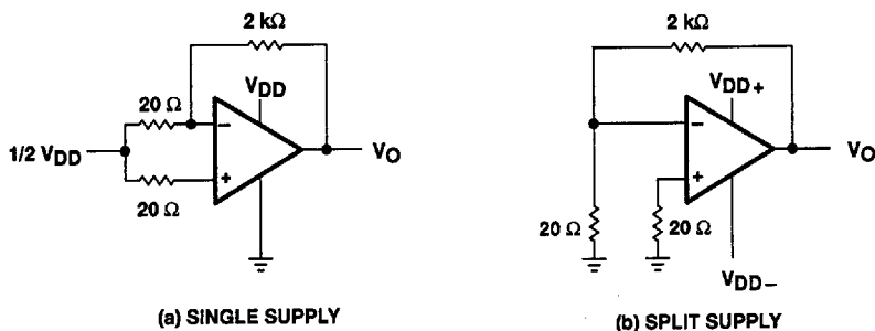
Figure 2. Noise-Test Circuit
