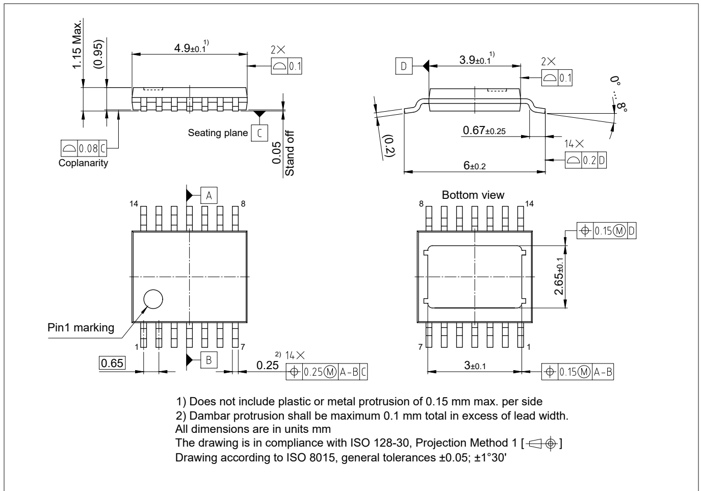
Figure 7 PG-TSDSO-14
