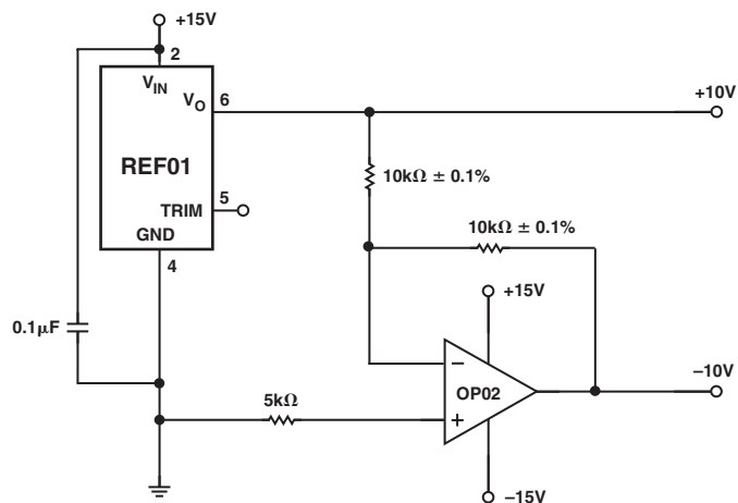
Figure 8. ±10 V Reference
