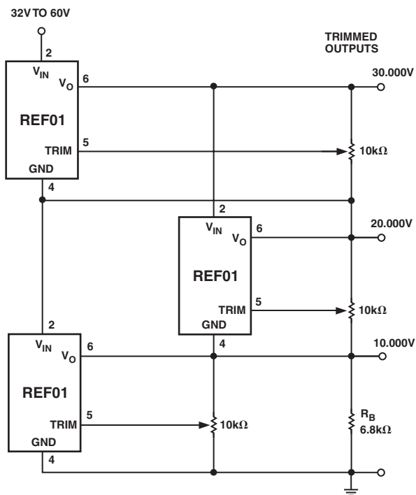
Figure 11. Reference Stack
