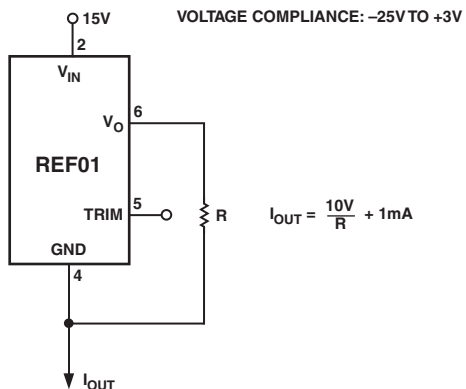
Figure 6. Current Source
