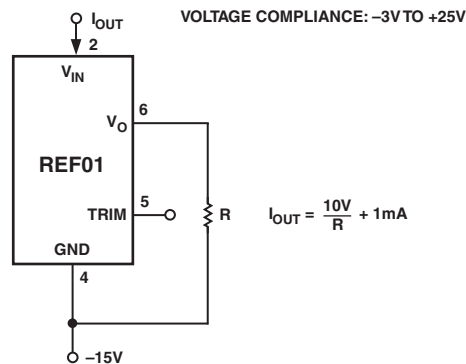
Figure 9. Current Sink
