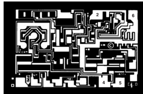
Figure 3. Dice Characteristics (125°C Tested Dice Available)
