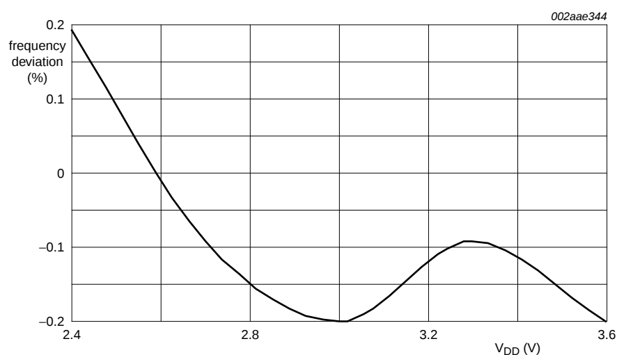
Fig 24. Average internal RC oscillator frequency vs. V_{DD} at +25 °C
