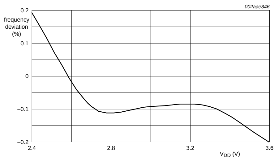
Fig 25. Average internal RC oscillator frequency vs. V_{DD} at -40 °C
