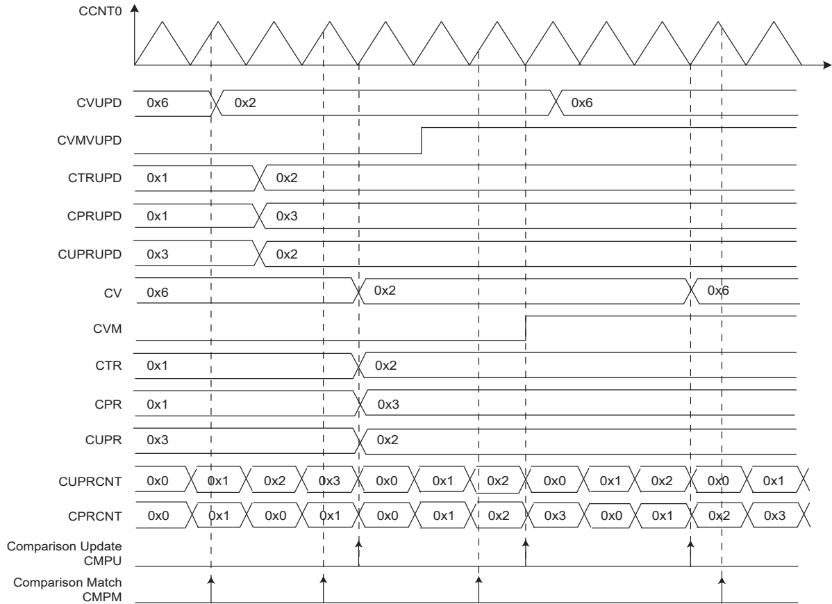
Figure 56-24. Comparison Waveform
