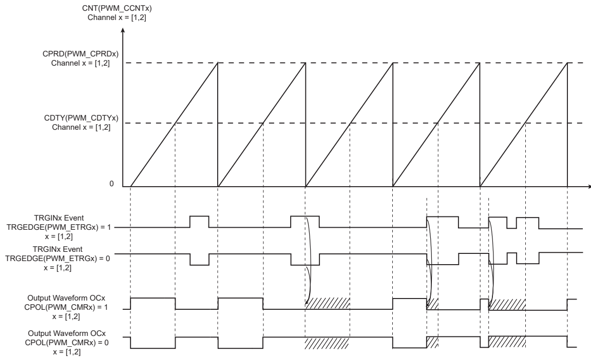
Figure 56-32. Cycle-By-Cycle Duty Mode
