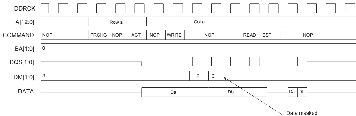
Figure 36-8. Single Write Access Followed by a Read Access, DDR2-SDRAM Devices
