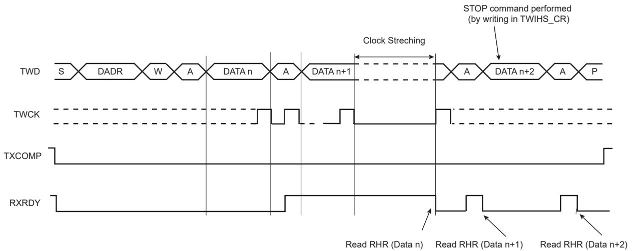
Figure 46-9. Host Read Clock Stretching with Multiple Data Bytes
