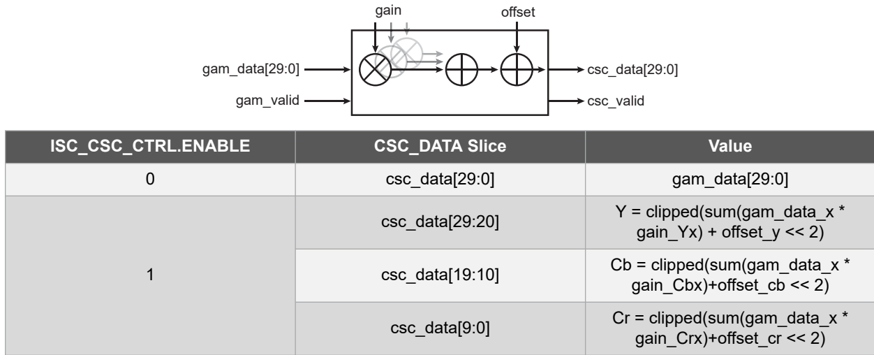
Figure 52-25. CSC Block Diagram
