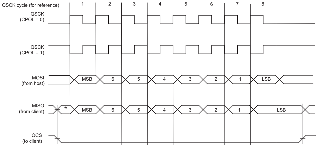
Figure 50-3. QSPI Transfer Format (QSPI_SCR.CPHA = 1, 8 bits per transfer), Mode 1 and 3
