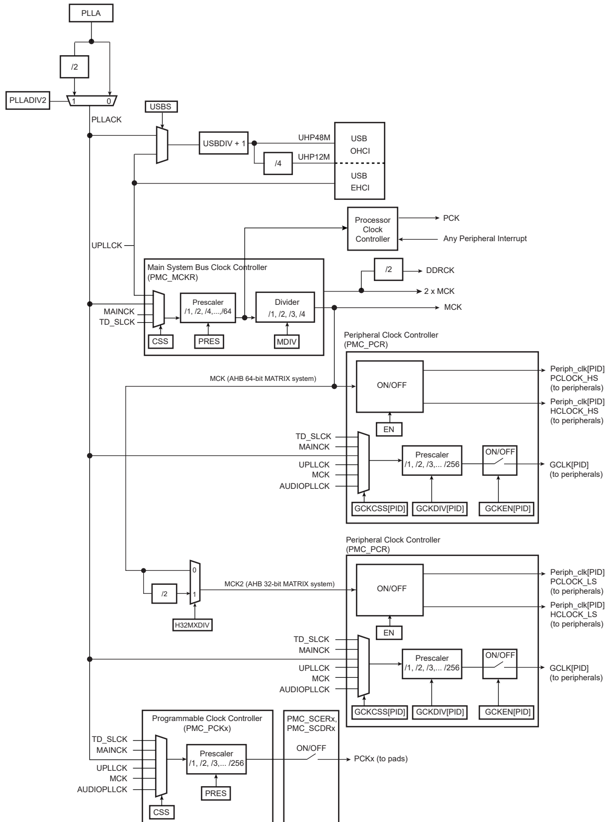
Figure 33-1. General Clock Block Diagram
