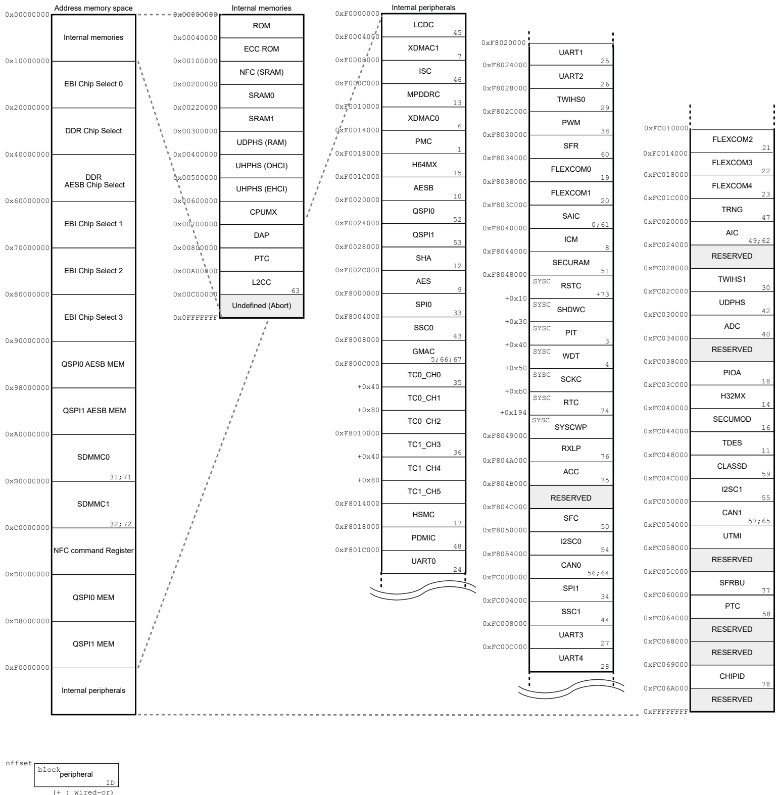
Figure 9-1. Memory Mapping
