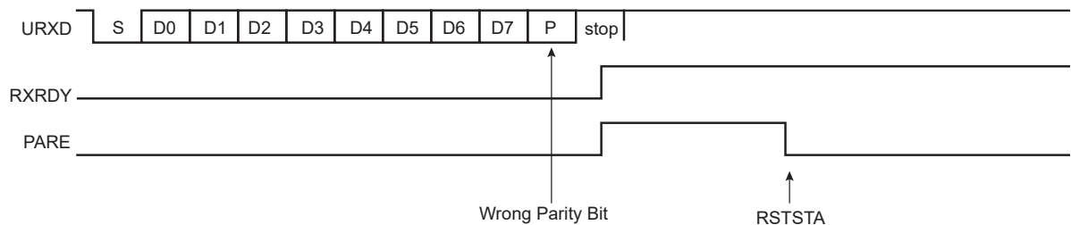
Figure 48-7. Parity Error
