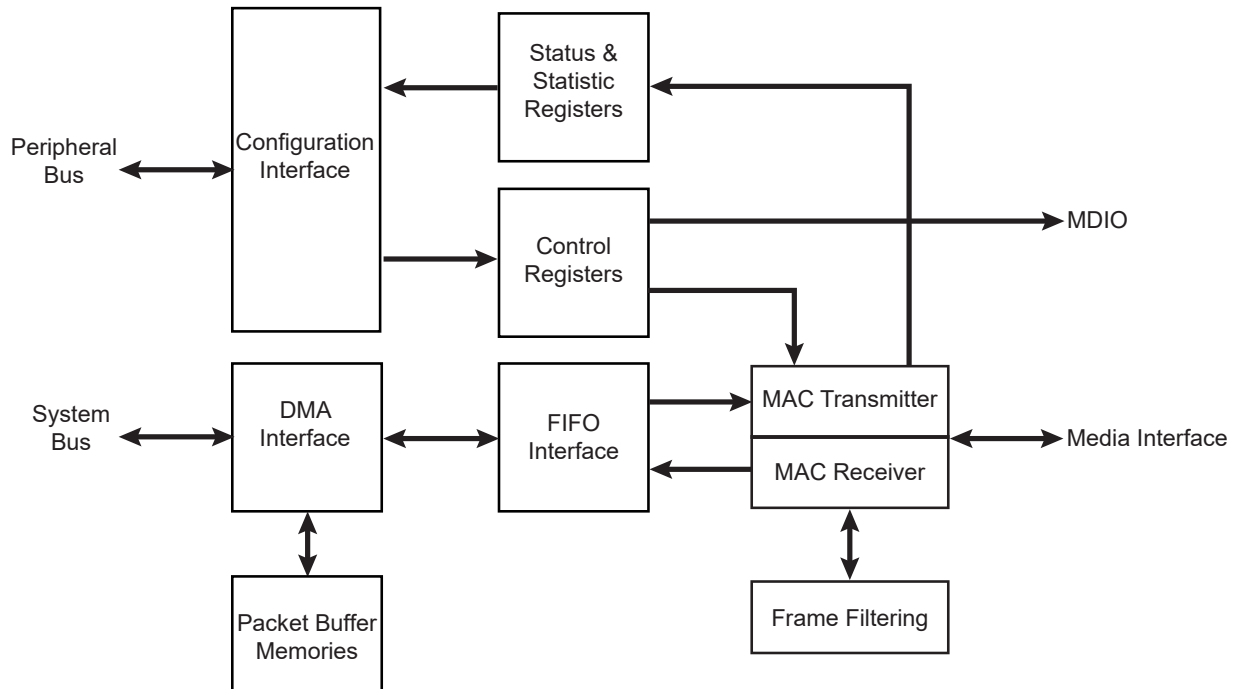
Figure 40-1. Block Diagram
