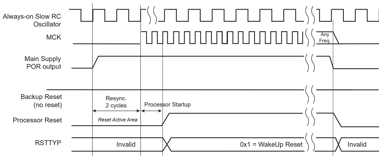
Figure 24-4. Wake-up Reset
