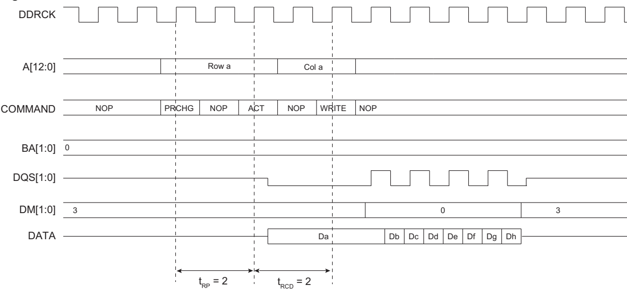
Figure 36-4. Burst Write Access, Row Closed, DDR-SDRAM Devices
