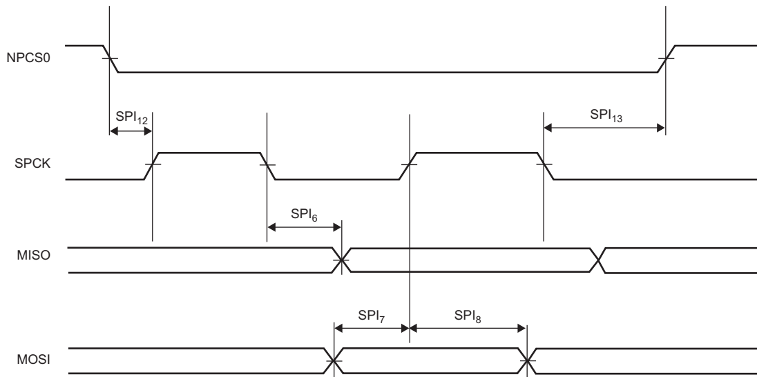
Figure 67-14. FLEXCOM in SPI Client Modes 0 and 3
