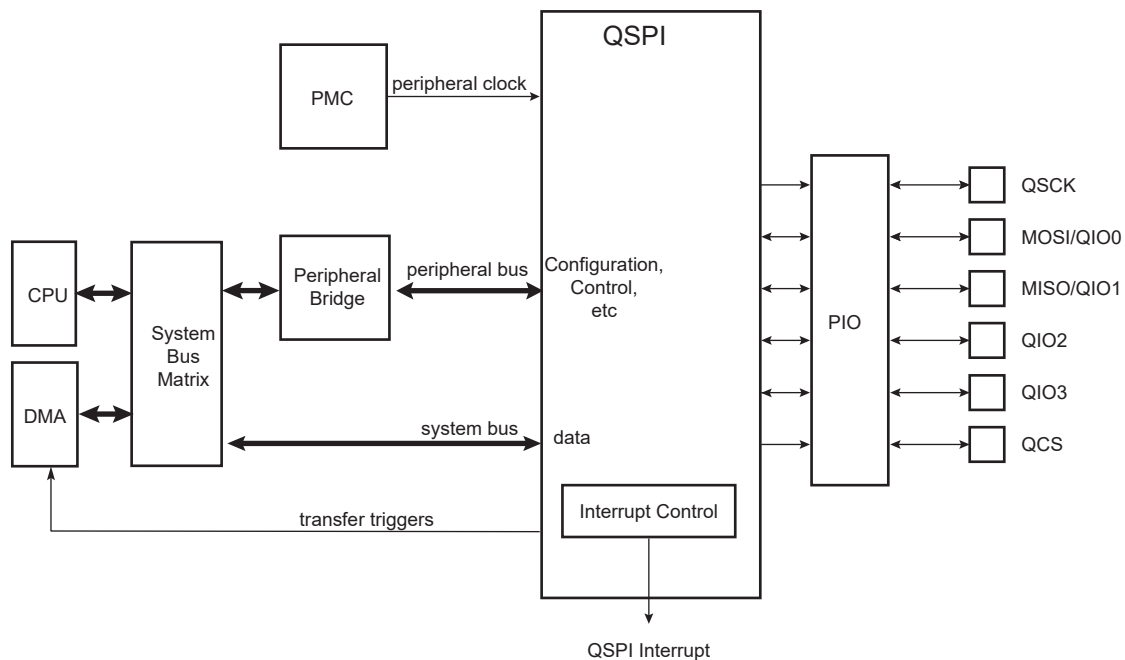
Figure 50-1. Block Diagram
