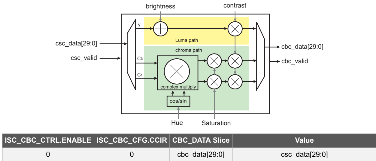
Figure 52-26. CBHS Block Diagram
