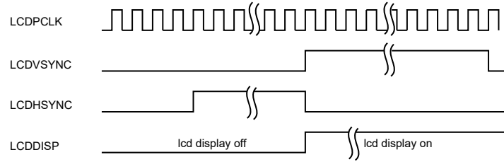
Figure 39-19. DISP Signal Timing Diagram
