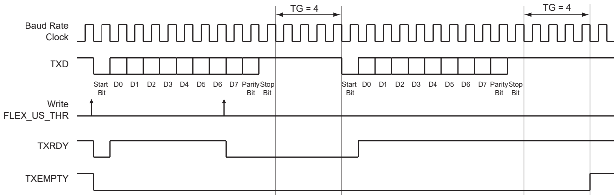
Figure 47-22. Timeguard Operations
