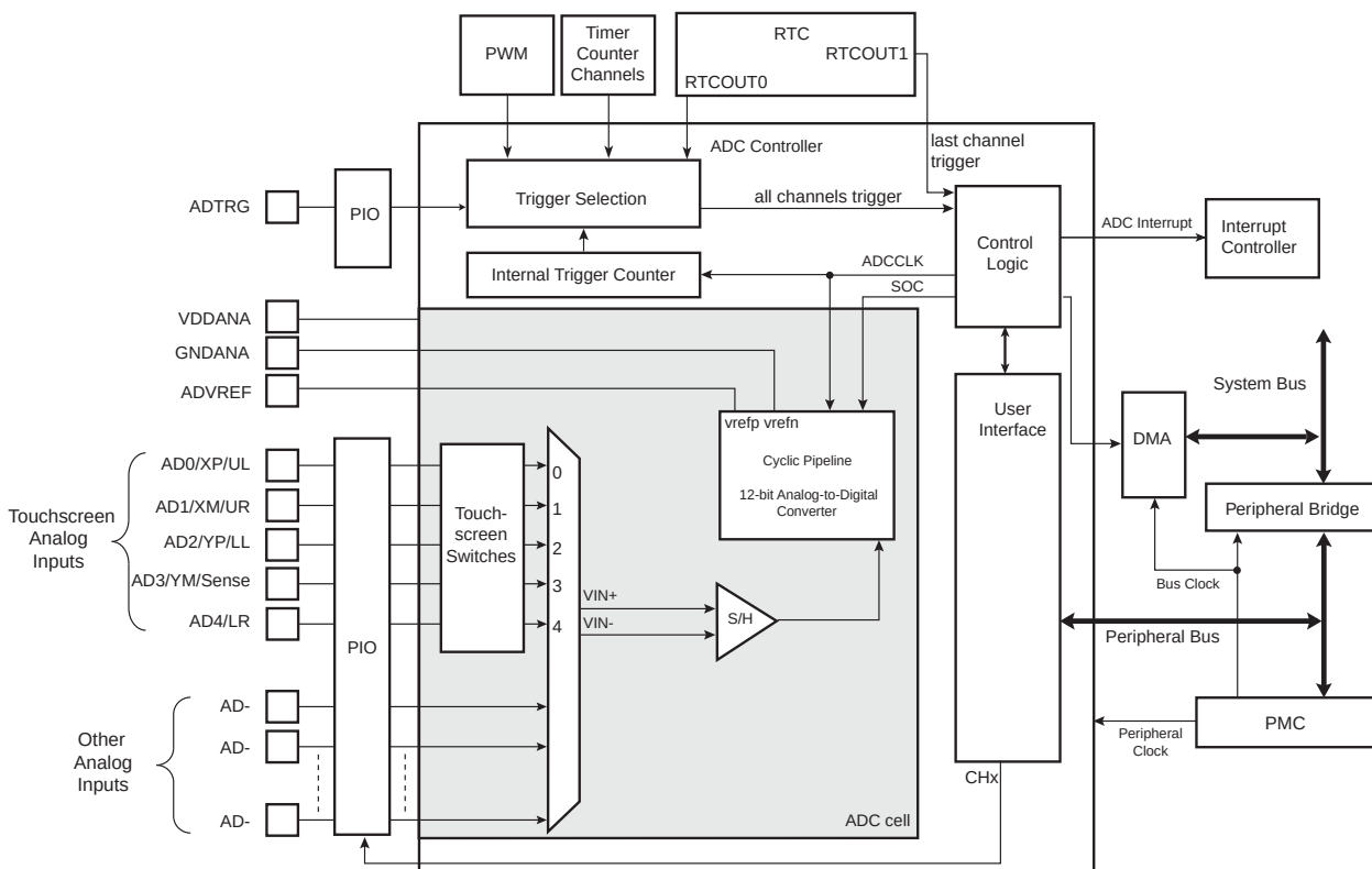
Figure 66-1. ADC Block Diagram
