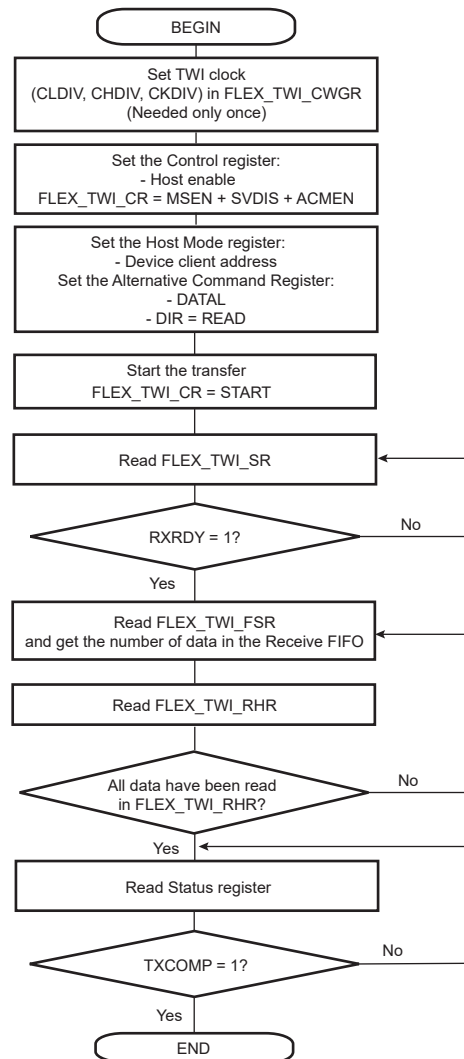
Figure 47-130. Receiving Data with FIFO Enabled in Host Mode
