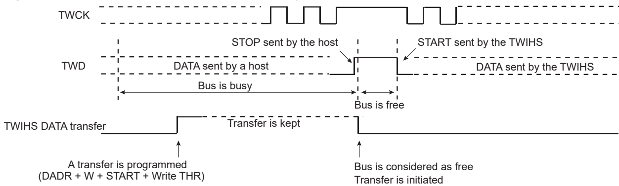
Figure 46-29. Arbitration Cases
