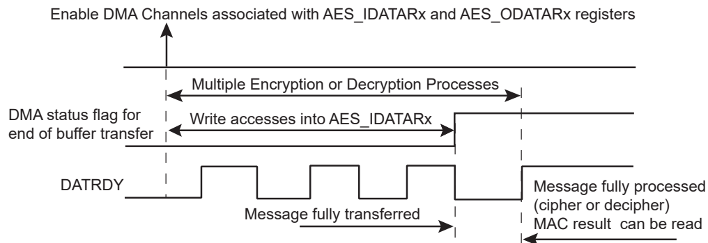
Figure 60-4. DMA Transfer with AES_MR.LOD = 1
