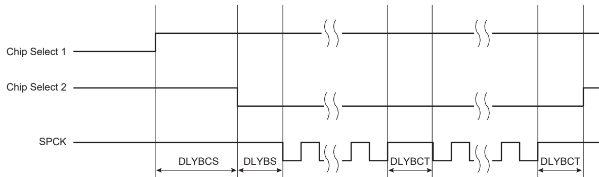
Figure 49-9. Programmable Delays
