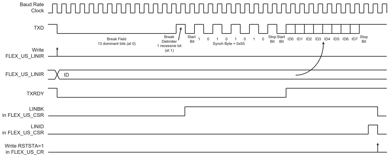
Figure 47-41. Header Transmission
