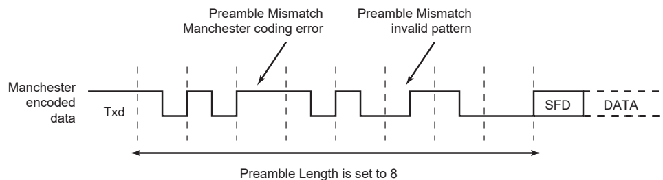
Figure 47-15. Manchester Error Flag
