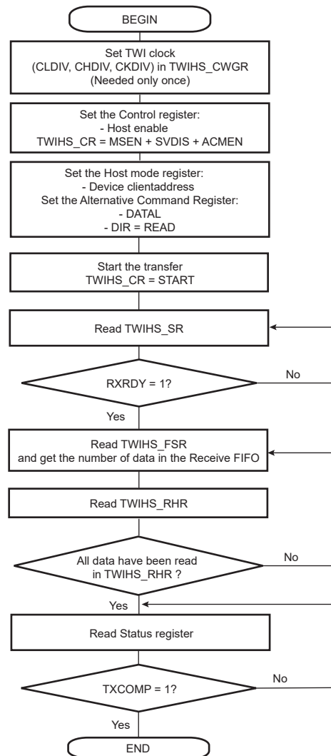
Figure 46-48. Receiving Data with FIFO Enabled in Host Mode
