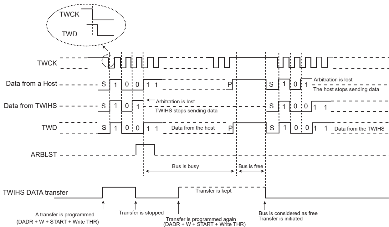
Figure 46-29. Arbitration Cases
