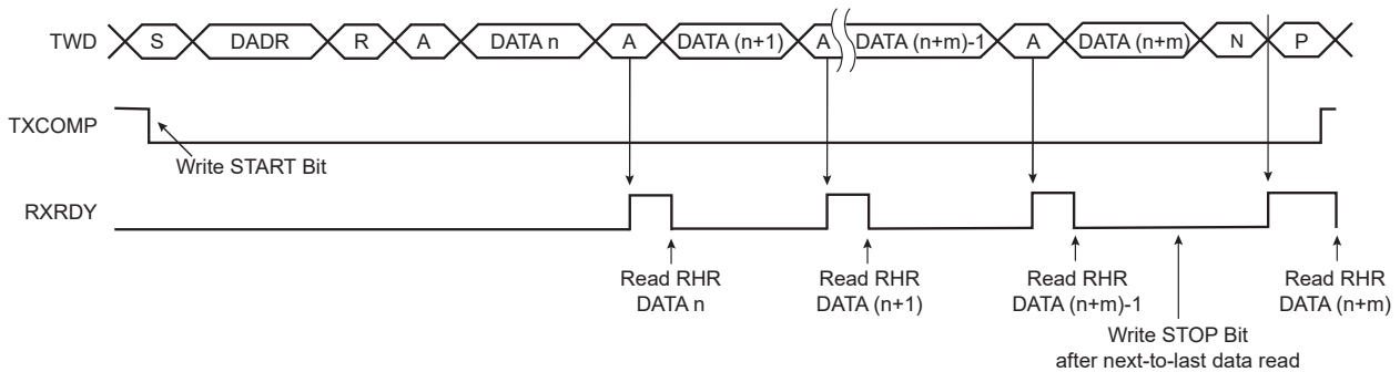
Figure 47-91. Host Read Clock Stretching with Multiple Data Bytes
