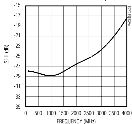
DIFFERENTIAL IS11 vs. FREQUENCY
