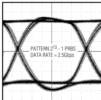
ELECTRICAL EYE DIAGRAM ( I_{MODQ} = 60\text{mA} )
