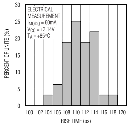
TYPICAL DISTRIBUTION OF RISE TIME (WORST-CASE CONDITIONS)
