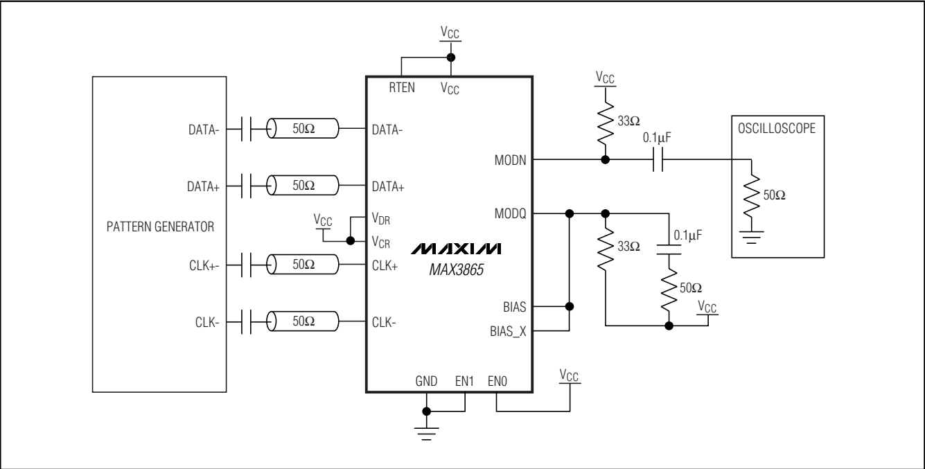
Figure 1. Test Circuit
