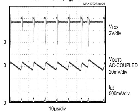
REG3 LIGHT-LOAD SWITCHING WAVEFORM LOAD = 10mA, V_{IN} = 4\text{V}
