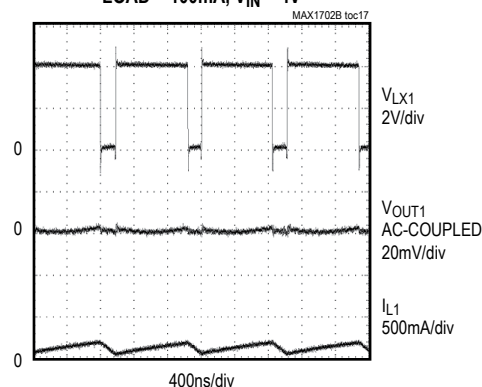
REG1 MEDIUM-LOAD SWITCHING WAVEFORM LOAD = 100mA, V_{IN} = 4\text{V}
