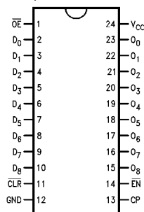
Pin Assignment for DIP, SOIC and TSSOP
