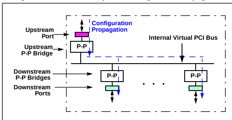
Figure 4-5. PEX 8609 System Configuration Propagation
