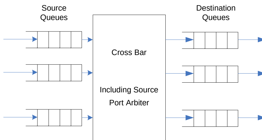
Figure 9-4. On-Chip Queuing
