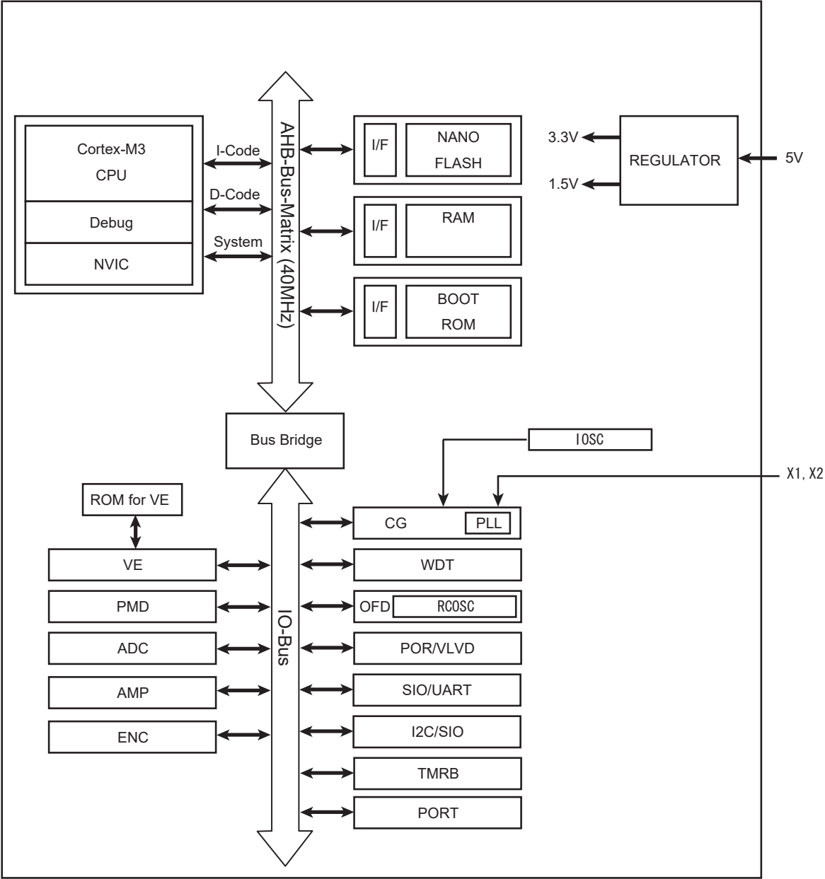
Figure 1-1 TMPM375FSDMG block diagram
