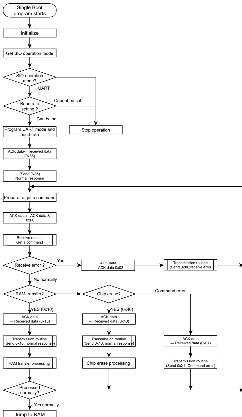
Figure 22-11 Boot program whole flowchart
