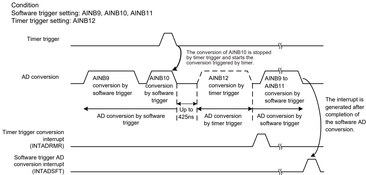
Figure 11-8 AD conversion by timer trigger
