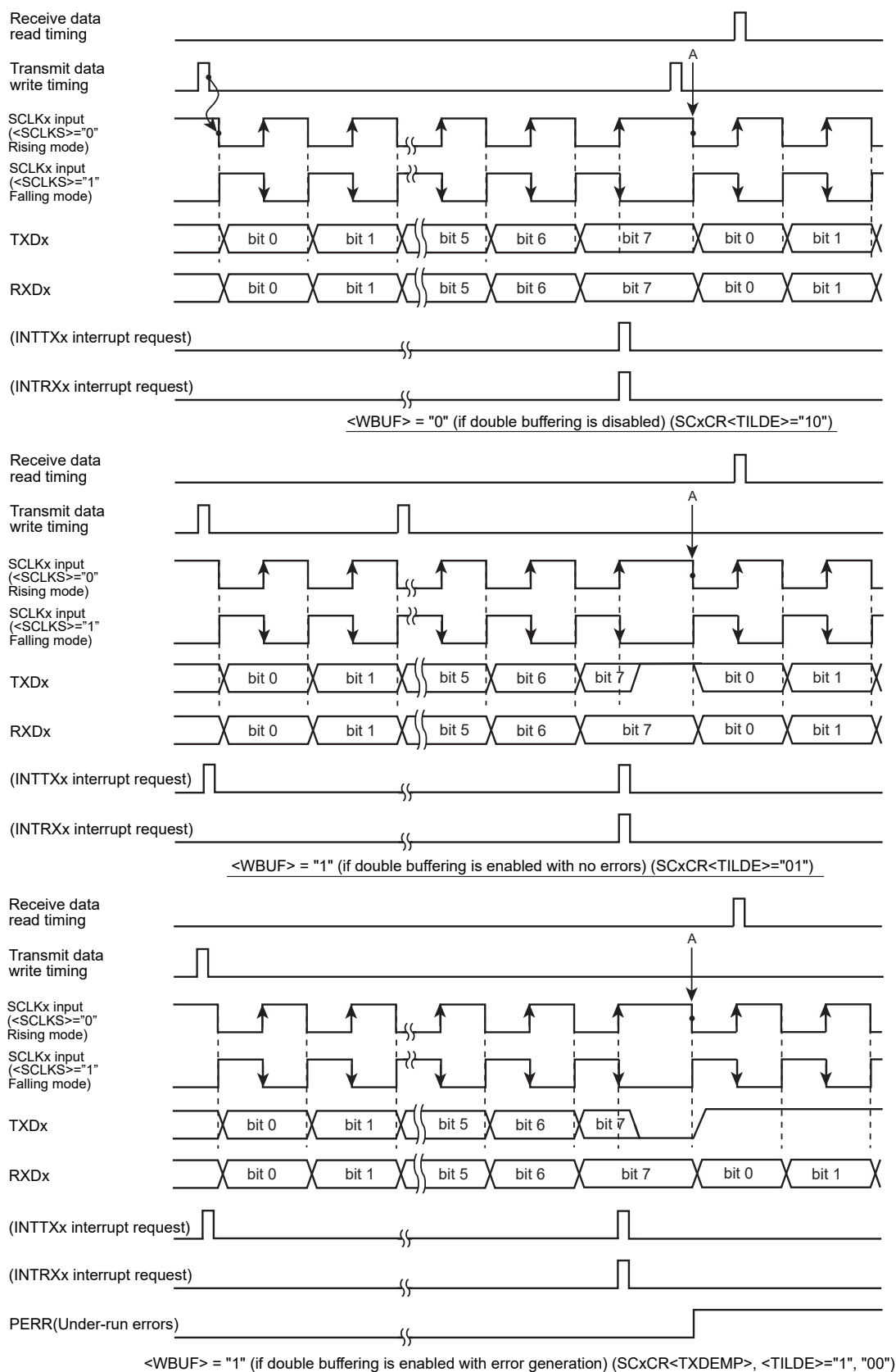
Figure 11-20 Transmit/Receive Operation in the I/O Interface Mode (SCLK Input Mode)
