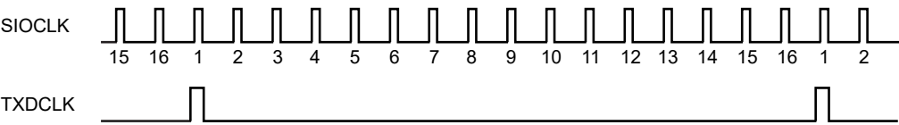
Figure 11-7 Generation of Transmission Clock
