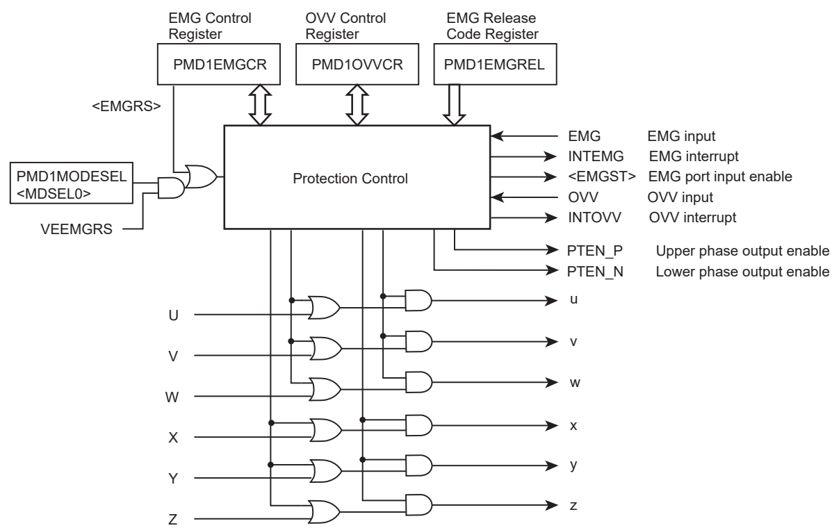
Figure 14-8 Protection Control Circuit
