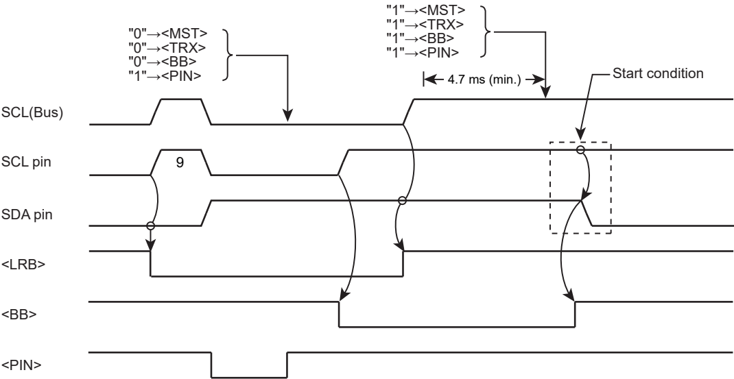
Figure 12-14 Timing Chart of Generating a Restart
