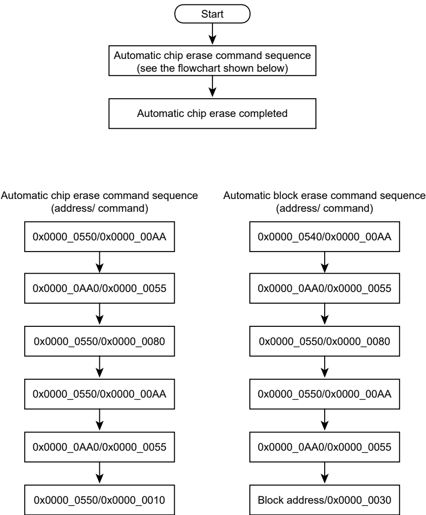
Figure 22-5 Flowchart of automatic erase
