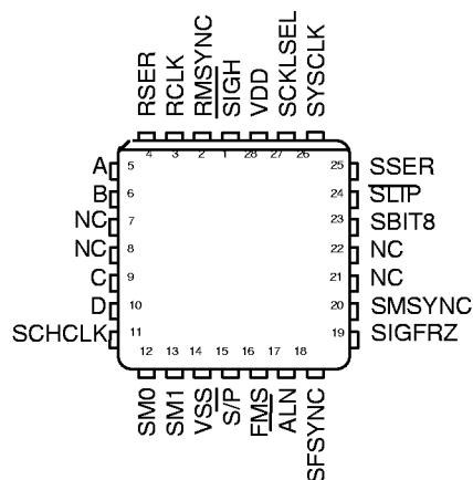
28-PIN PLCC
