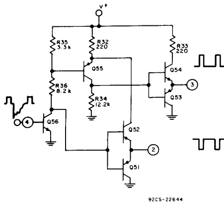
Fig. 3 - Sync separator stage.
