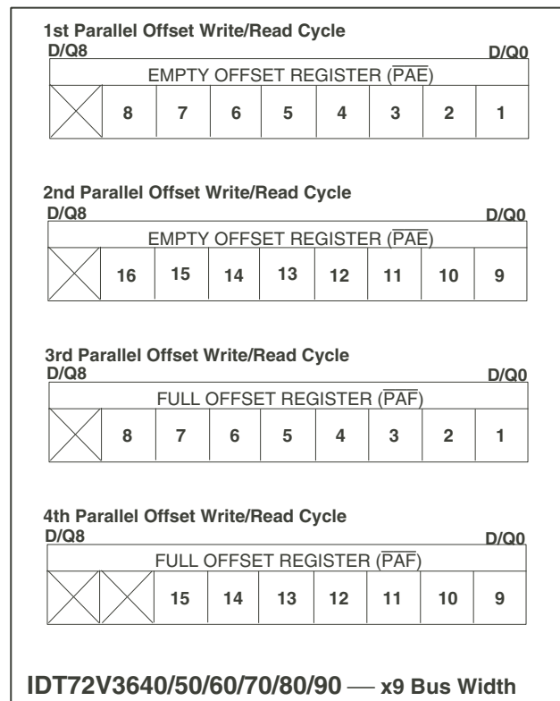
Figure 3. Programmable Flag Offset Programming Sequence (Continued)
